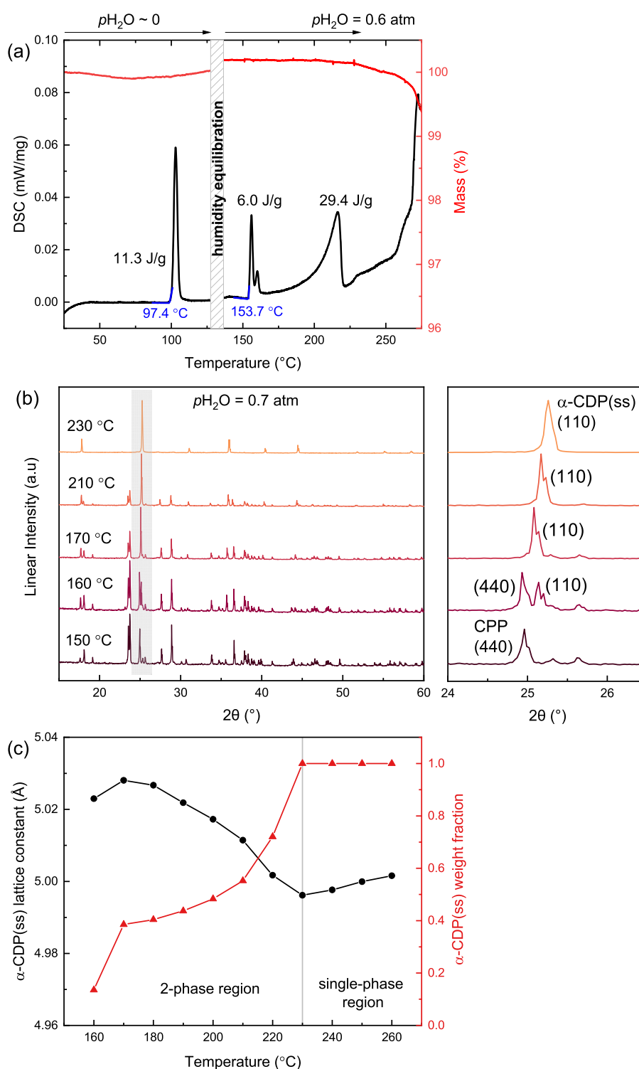
Figure 6. Phase transformation behavior of (1-x)\text{CsH}_2\text{PO}_4 - x\text{H}_3\text{PO}_4 at x = 0.07 : (a) Simultaneously measured TGA/DSC profiles at a heating rate of 1 ^{\circ}\text{C}/\text{min} ; (b) XRD patterns measured at the temperatures indicated; and (c) lattice constant and weight fraction as functions of temperature (uncertainties in the refined values fall within the span of the datapoint symbols). (a) p\text{H}_2\text{O} = 0.6 \text{ atm} (balance Ar) was introduced at 130 ^{\circ}\text{C} as part of the heating protocol, and data reflecting system equilibration to the high-humidity condition are omitted. (b) Sample chamber atmosphere maintained at p\text{H}_2\text{O} = 0.7 \text{ atm} (balance \text{N}_2 ). (c) Lines between points serve only to guide the eye and do not reflect sample behavior between measurement temperatures. The results reveal the transitions \text{CDP(m)} + \text{CsH}_5(\text{PO}_4)_2 \rightarrow \text{CDP(m)} + \text{CPP} @ 90 ^{\circ}\text{C} and \text{CDP(m)} + \text{CPP} \rightarrow \text{CDP(m)} + \alpha\text{-CDP(ss)} @ 160 ^{\circ}\text{C} .
