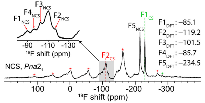
FIG. 4. High-resolution ^{19}\text{F} MAS (25 kHz) NMR spectrum of NCS \text{Pna2}_1 \text{KNaNbOF}_5 and its calculated ^{19}\text{F} NMR chemical shifts shown for reference. Asterisks (*) denote spinning side bands. ^{19}\text{F} MAS (25 kHz) NMR spectrum of CS \text{P4}/\text{mmm} \text{KNaNbOF}_5 is shown in Fig. S6 for comparison.
