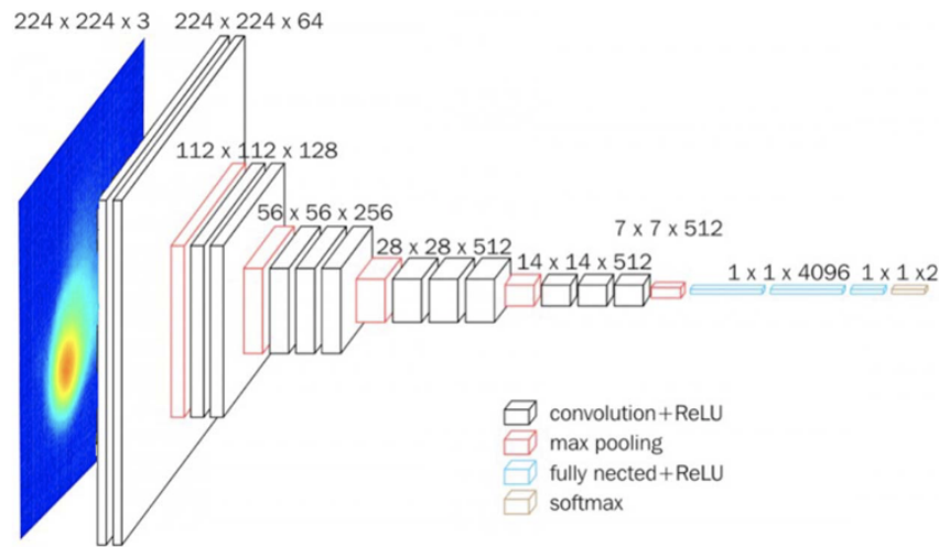
Figure 3. The VGG16 architecture modified for the PyroNet [22].
