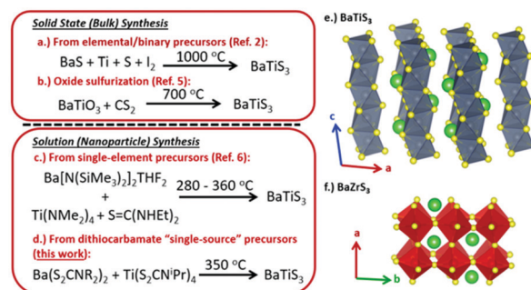
Fig. 1 (a–d) Synthetic approaches to BaTiS 3 in the bulk and as nanocrystals. (e) Structure of hexagonal BaTiS 3 . (f) Structure of BaZrS 3 , an example of a chalcogenide perovskite.
