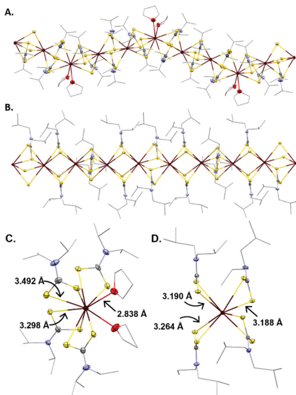
Fig. 2 Crystal structures of barium dithiocarbamate complexes 1 (A) and 2 (B). Hydrogen atoms are omitted and, for clarity, carbons in alkyl groups are represented in wireframe. Other atoms are shown as thermal ellipsoids at 50% probability. Both structures are truncated sections of one-dimensional coordination polymers. Panels (C) and (D) show magnified views of the coordination environments around the 10-coordinate \text{Ba}^{2+} ion in 1 (C) and one of the 8-coordinate \text{Ba}^{2+} ions in 2 (D), along with selected bond distances. (Red = O; yellow = S; maroon = Ba; purple = N; gray = C).
