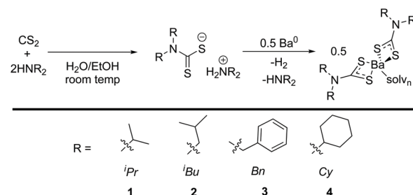
Scheme 1 Synthesis of barium dithiocarbamate precursors.
