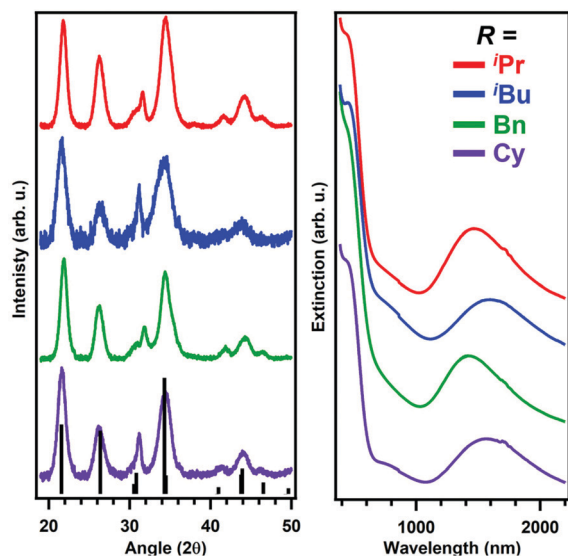
Fig. 3 Characterization of BaTiS 3 nanocrystals synthesized using the standard conditions described in the text with barium dithiocarbamate precursors Ba(S 2 CNR 2 ) 2 with different substituents (R). (Left) Powder X-ray diffraction data for BaTiS 3 nanocrystals (normalized and offset for clarity); reference BaTiS 3 pattern is shown along the bottom (black lines). Colors correspond to the legend shown in the top right. (Right) UV-Vis-NIR spectra (normalized and offset for clarity) of suspensions of the BaTiS 3 nanocrystals in tetrachloroethylene.
