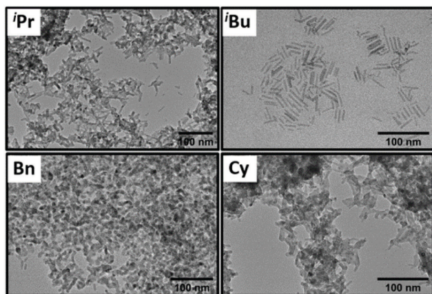
Fig. 4 TEM images of BaTiS 3 nanocrystals synthesized using different precursors. The samples show varying degrees of aggregation during sample preparation.
