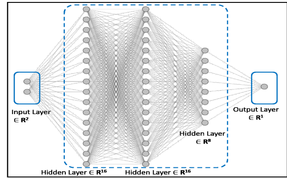
Figure 3: Structure of the deep learning model used for the training, testing and validating of the processed data.
