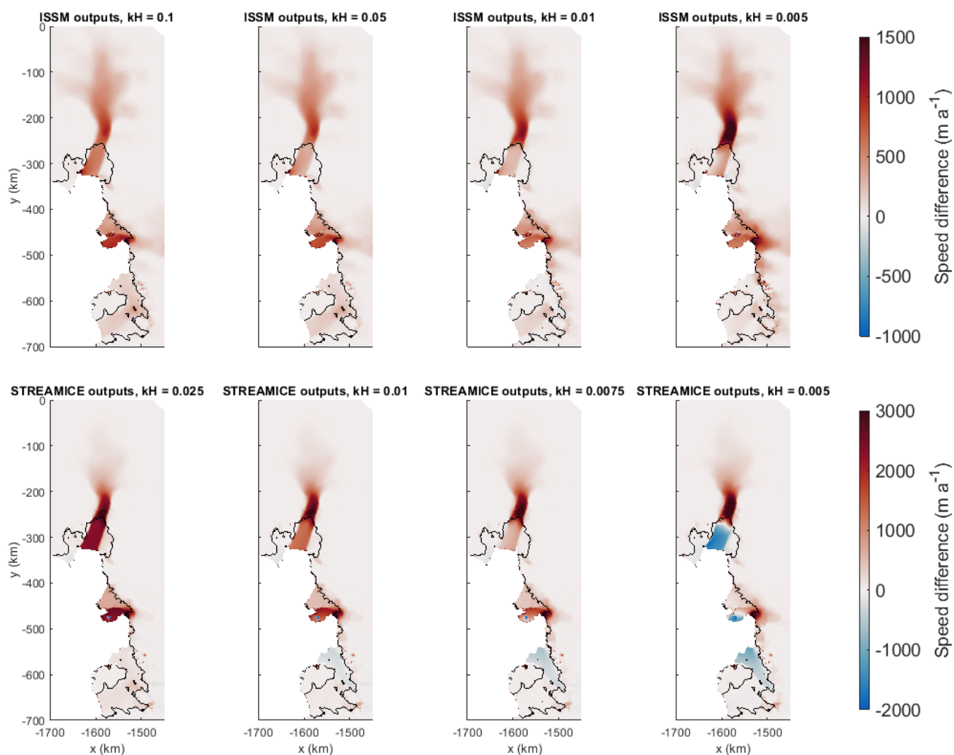
Figure C2. Differences between diagnostic speeds calculated in \dot{U}_a using the ISSM and STREAMICE inversion outputs and a range of values for kH and the speeds calculated in the original models. Note that each row uses a different colour scale.
