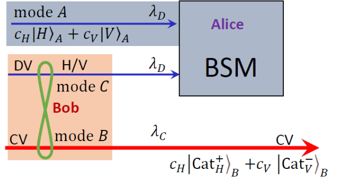
Figure 3. (color online) Schematic of teleporting an unknown single-photon polarization qubit via hybrid DV-CV quantum entanglement.
