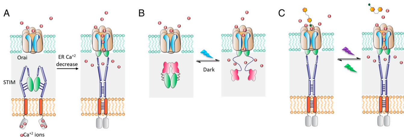
Fig. 1. CRAC channel activation and photocontrol. (A) Depletion of ER \text{Ca}^{2+} causes STIM aggregation and activation of CRAC channels by binding to Orai. (B) Opto-CRAC provides photocontrol of \text{Ca}^{2+} -dependent events through a fusion construct of the STIM1–Orai1-activating region (SOAR) domain and plant-derived photosensory light-activated voltage domain 2 (LOV2). (C) Use of the azobenzene-based photoswitch LOCI enables control of native CRAC channel activity using UV and visible light.
