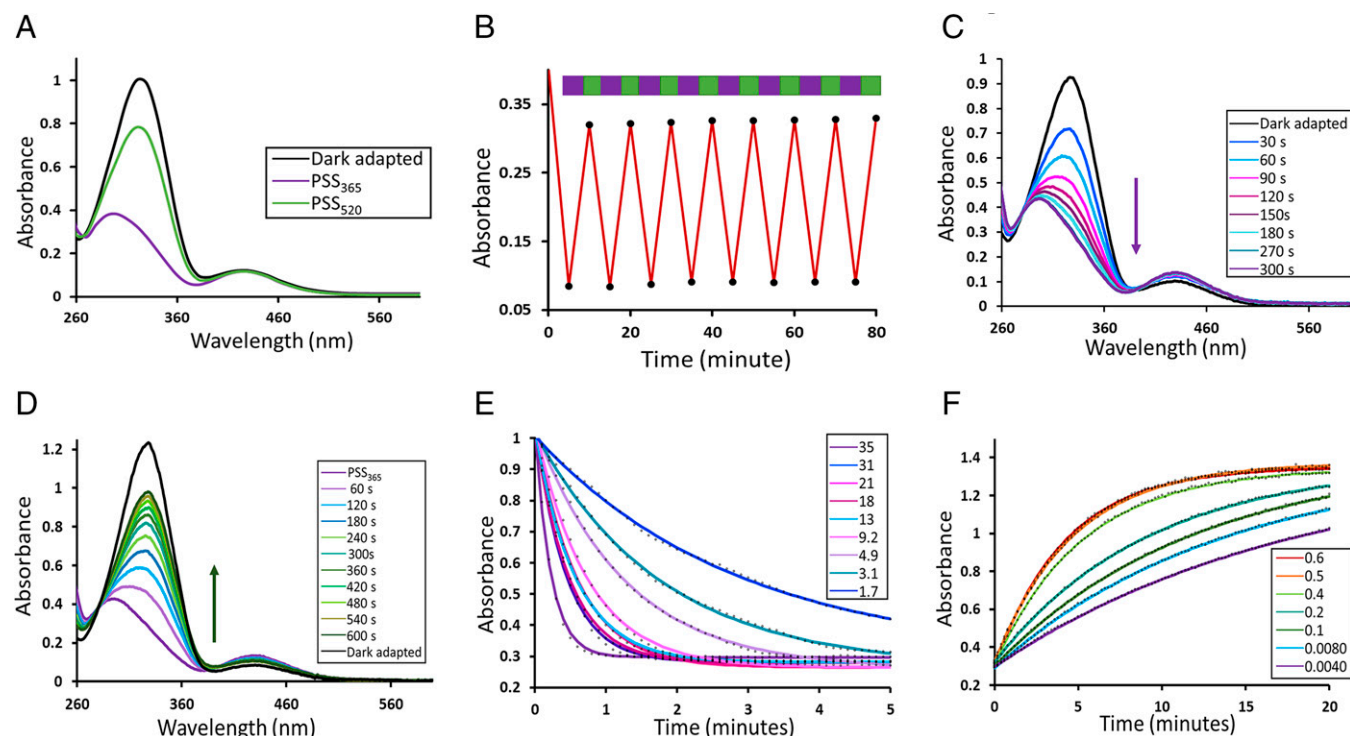
Fig. 2. Photochemical characterization of LOCI-1. (A) UV/Vis absorption spectra of LOCI-1 (22 \mu M) in DMSO, with dark-adapted (black), photostationary state with 365 nm LED illumination PSS 365nm (purple) and PSS 520nm (green) states when irradiated with UV and green light for 5 min, respectively. (B) Photostability of LOCI-1 (26 \mu M) in a 1% DMSO in PBS buffer solution. Absorbance changes recorded at 329 nm under alternating 5-min light illumination of 365 nm (purple) and 520 nm (green) for eight cycles. (C and D) Time-resolved UV/Vis spectra of LOCI-1 (23 \mu M) during irradiation with 365 nm and 520 nm LEDs, respectively. (E and F) Absorbance of LOCI-1 (23 \mu M) monitored at 329 nm upon illumination with a high power 365-nm light source (Omnicure S1000 100 W mercury arc lamp) and a 520-nm LED at different irradiation powers, measured in mW/cm^2 .
