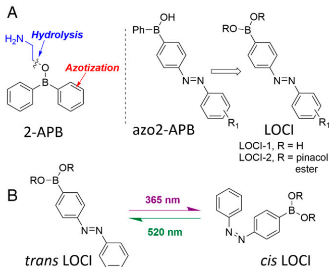
Scheme 1. 2-APB structure–activity relationships informed the design of LOCI. (A) “Azotization” of 2-APB through intermediate LOCI with either the free boronic acid (LOCI-1) or pinacol ester (LOCI-2). (B) Trans LOCI-1 can be efficiently isomerized to the cis isomer using UV light (365 nm) and switched back to the trans isomer using green light (520 nm).
