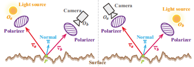
Figure 1. Configuration of the polarimetric Helmholtz stereopsis.
