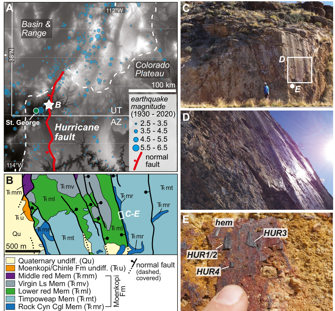
Figure 1. (a) Digital elevation model with the Hurricane fault and 1930–2020 earthquake catalog; blue circles scaled to earthquake magnitude. White star denotes study area. (b) Simplified geologic map modified from Biek (2003). White box is (c–e) location. (c–d) Field photographs of targeted, mirrored fault surface; (e) hematite patches.
