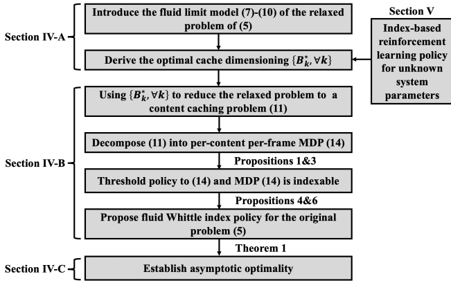
Fig. 1: The framework of the proposed solution.
