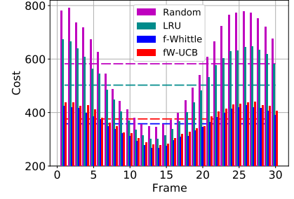
Fig. 4: Comparison of costs.
