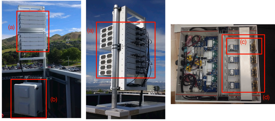
Fig. 7. mMIMO base station: (a) Radio and antenna array, (b) Hub, (c) 2 \times 2 Transceiver and antenna, (d) Transceiver chain.
