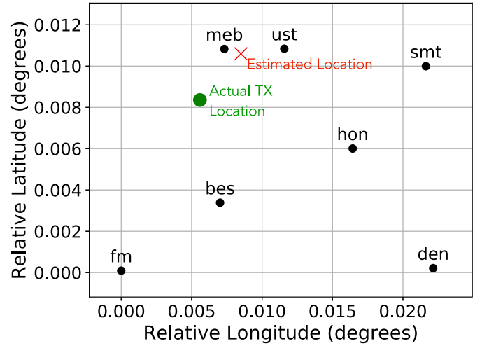
Fig. 19. Actual and estimated location of transmitter from an example localization experiment.
