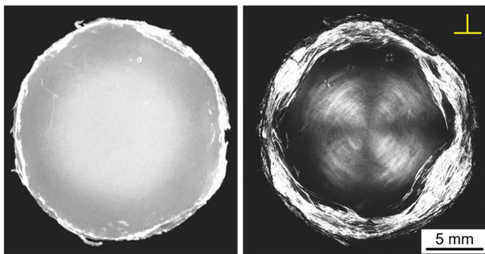
Fig. 4 Photograph (left) and POM image (right) of a PA 11 disk crystallized at 180^\circ\text{C} for 1 h after shearing the melt at 7.6 \text{ s}^{-1} for 60 s, taken at room temperature. The orientation of the polarizers is shown at the top right of the POM image
