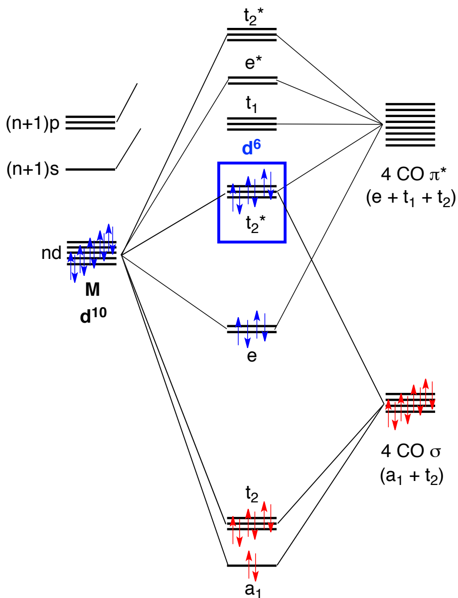
Figure 14. Qualitative molecular orbital diagram for [M(CO)_4]^Q compounds with an 18-electron configuration, in which backbonding is considered to be significant e.g. [Fe(CO)_4]^{2-} . Note that the occupied e -set of bonding orbitals are not included in the formally nonbonding d^n configuration if there is significant backbonding.
