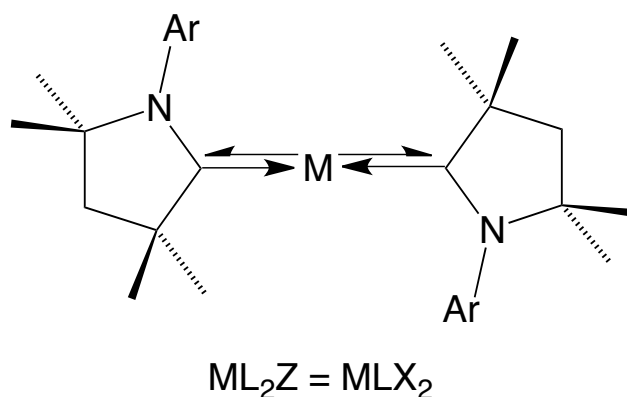
Figure 17. CBC representation of (\text{cAAC}^{\text{Ar}})_2\text{M} . The 3c-2e \pi -interaction is represented with two “half-arrows” which indicate that the pair of electrons is donated to both carbon atoms.
