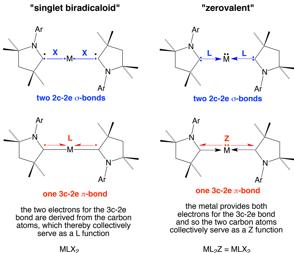
Figure 16. Demonstration that the “singlet biradicaloid” and “zerovalent” descriptions of (\text{cAAC}^{\text{Ar}})_2\text{M} are equivalent according to the CBC method. For each description, the upper figure illustrates the two 2c-2e \sigma -bonds, while the bottom figure illustrates the 3c-2e \pi -bond.
