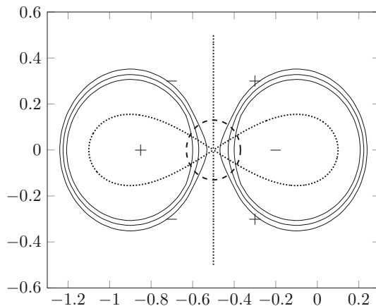
Fig. 5 Illustration of the contours when \alpha = 1 . The dotted lines represent the level curve \text{Re}h(w) = \text{Re}h(w_c) . It consists of two closed contours and one infinite contour all of which pass the critical point w_c . The complex plane thus is split into four parts, two of them marked with - signs have lower levels of \text{Re}h(w) , and the other two marked with + signs have higher levels of \text{Re}h(w) . The three solid contours on the left, from inside to outside, are \Sigma_{L,\text{in}} , \Sigma_L , \Sigma_{L,\text{out}} respectively. The three solid contours on the right, from inside to outside, are \Sigma_{R,\text{in}} , \Sigma_R , and \Sigma_{R,\text{out}} respectively. Each contour \Sigma_* is split into two parts. The part within the dashed circle is \Sigma_*^{(N)} , and the remaining part is \Sigma_*^{(\text{err})}
