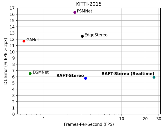
Figure 6. Plot comparing zero-shot generalization from synthetic data to KITTI-2015. All methods are trained only on Sceneflow [23], without any fine-tuning. RAFT-Stereo can be configured for real time inference and achieves competitive performance with the state-of-the-art stereo methods. Relative to our base model (blue), our realtime model (teal) uses a shared backbone, two hidden state resolutions and slow-fast GRUs updating the flow-field at 1/8th resolution (Sec. 4.7)
