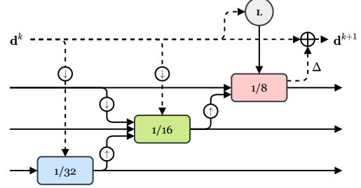
Figure 3. Multilevel GRU. We use a 3-level convolutional GRU which acts on feature maps at 1/32, 1/16, and 1/8 the input image resolution. Information is passed between GRUs at adjacent resolutions using upsampling and downsampling operations. The GRU at the highest resolution (red) performs lookups from the correlation pyramid and updates the disparity estimate.
