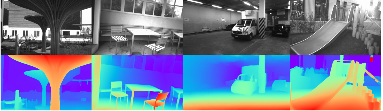
Figure 4. Results on the ETH3D stereo dataset. RAFT-Stereo is robust to difficulties like textureless surfaces and overexposure.
