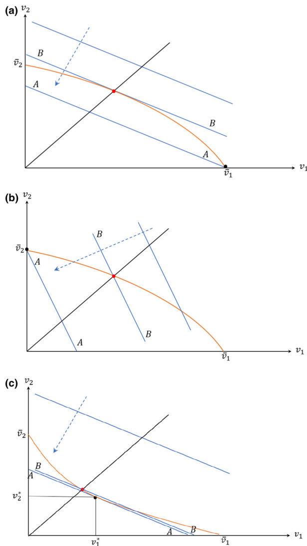
Fig. 1 Vaccination threshold values for group 1 and group 2. The orange curve shows values of vaccination coverage where the vaccinated reproductive number is equal to one: \mathcal{R}_v = 1 . The slope of this curve when intersects with the y-axis is given by -\frac{\varepsilon_1 \mathcal{R}_{12} \mathcal{R}_{21}}{\varepsilon_2 (\mathcal{R}_{22} + \mathcal{R}_{12} \mathcal{R}_{21} - \mathcal{R}_{11} \mathcal{R}_{22})^2} . The blue level curves show different values of total vaccination coverage going down in the direction of the origin: n_1^* v_1^* + n_2^* v_2^* . The slope of these level curves is -\frac{n_1^*}{n_2^*} . Under biased random mixing (a) when the blue line is flatter than the orange curve when it intersects the y-axis, the closest blue line to the origin that intersect the orange curve occurs when v_1^* = \bar{v}_1 = \frac{\mathcal{R}_{11} + \mathcal{R}_{22} + \mathcal{R}_{12} \mathcal{R}_{21} - \mathcal{R}_{11} \mathcal{R}_{22} - 1}{\varepsilon_1 (\mathcal{R}_{11} + \mathcal{R}_{12} \mathcal{R}_{21} - \mathcal{R}_{11} \mathcal{R}_{22})} , v_2^* = 0 ; (b) when the blue line is steeper than the orange curve when it intersects the x-axis, the closest blue line to the origin that intersect the orange curve occurs when v_1^* = 0 , v_2^* = \bar{v}_2 = \frac{\mathcal{R}_{11} + \mathcal{R}_{22} + \mathcal{R}_{12} \mathcal{R}_{21} - \mathcal{R}_{11} \mathcal{R}_{22} - 1}{\varepsilon_2 (\mathcal{R}_{22} + \mathcal{R}_{12} \mathcal{R}_{21} - \mathcal{R}_{11} \mathcal{R}_{22})} . Under biased assortative mixing (c) the optimum occurs when the blue line is tangent to the orange curve. In the homogeneous population model ( v_1^* = v_2^* ), the optimum occurs at the intersection of the black 45-degree line with the orange curve
