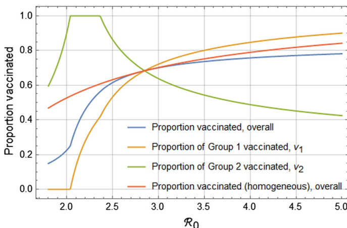
Fig. 3 Vaccine coverage above which herd immunity is achieved by group and basic reproduction number. Parameters values: \mathcal{R}_{12} = 1.0 , \mathcal{R}_{21} = 0.8 , \mathcal{R}_{22} = 1.3 , \varepsilon = 0.95 , \varepsilon_1 = 0.95 , \varepsilon_2 = 0.95 , N_1^* = 0.75 , N_2^* = 0.25 . Using the definition of \mathcal{R}_0 , we chose \mathcal{R}_{11} = (\mathcal{R}_0^2 - \mathcal{R}_{12}\mathcal{R}_{21} - \mathcal{R}_0\mathcal{R}_{22})/(\mathcal{R}_0 - \mathcal{R}_{22}) .
