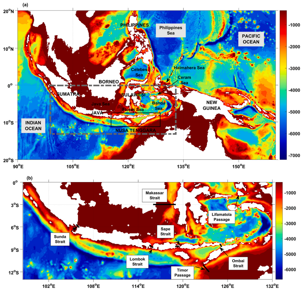
Fig. 1. (a) The 0.08° global HYCOM topography (m) for the Indonesian Seas. (b) The dashed grey boxed inset shows straits where the ITF transport is calculated. The solid black boxed inset denotes the Nusa Tenggara islands.
