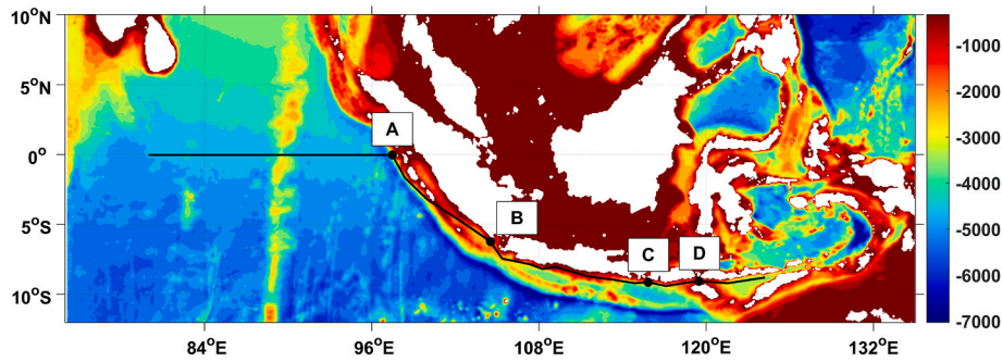
Fig. 14. Chosen path (black solid line) for the calculation of the Hovmöller diagram on top of 1/12° global HYCOM topography (m). The path is also featured on Figs. 12 and 13 upper right panel as a solid green line.
