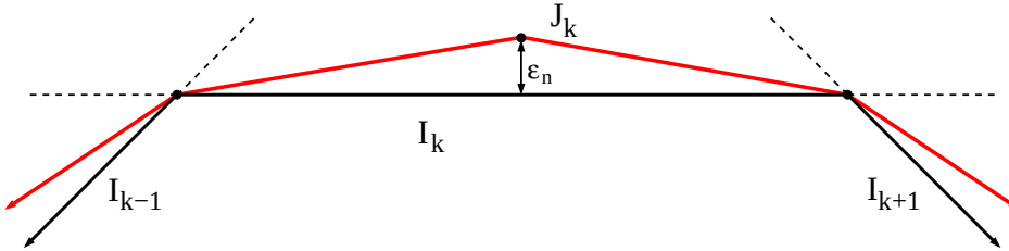
Figure 4: Constructing K_{n+1} from K_n to give a strictly convex example.
