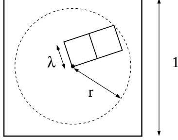
Figure 2: The center of a unit cube in Z_0 is contained in a \lambda -sized cube in \lambda\tau(Z_0) and we either keep that cube or an adjacent one. In either case the kept cube is contained in disk of radius r = \lambda\sqrt{d+3} around the center and hence it is inside the unit cube if \lambda \leq 1/(2\sqrt{d+3}) . This holds even if the cubes come from grids that are rotated with respect to each other.
