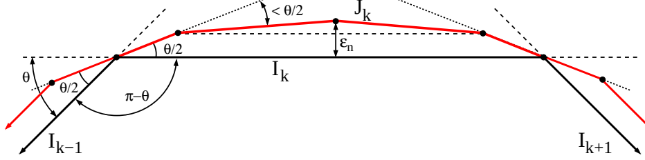
Figure 5: Constructing K_{n+1} from K_n to give a C^1 boundary in the limit.
