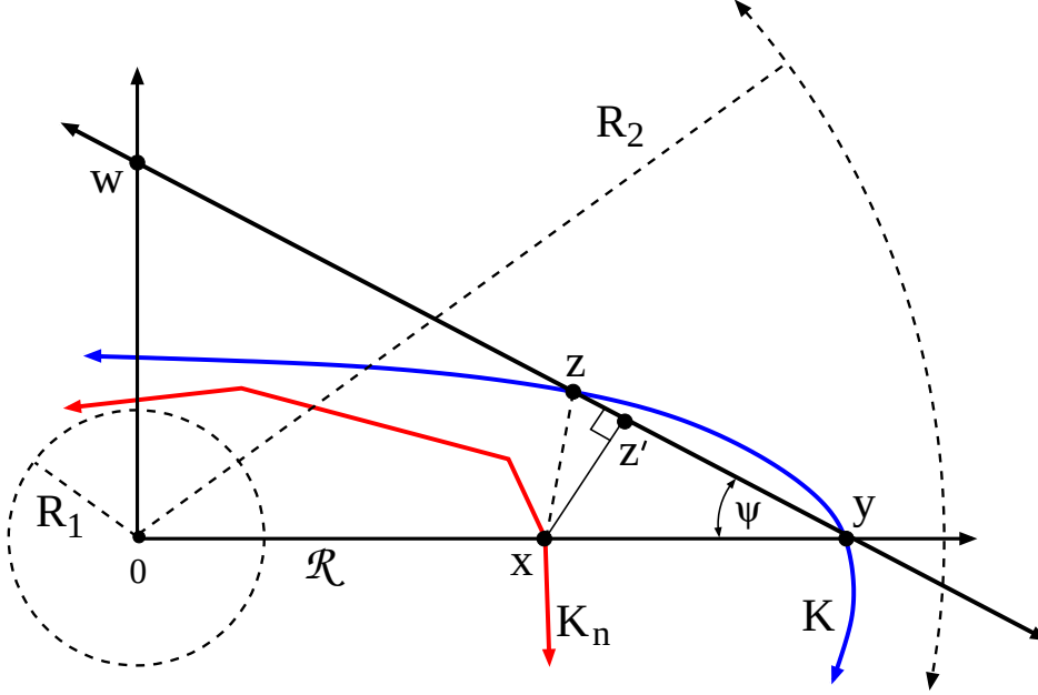
Figure 3: Illustration of the proof of Claim 1.
