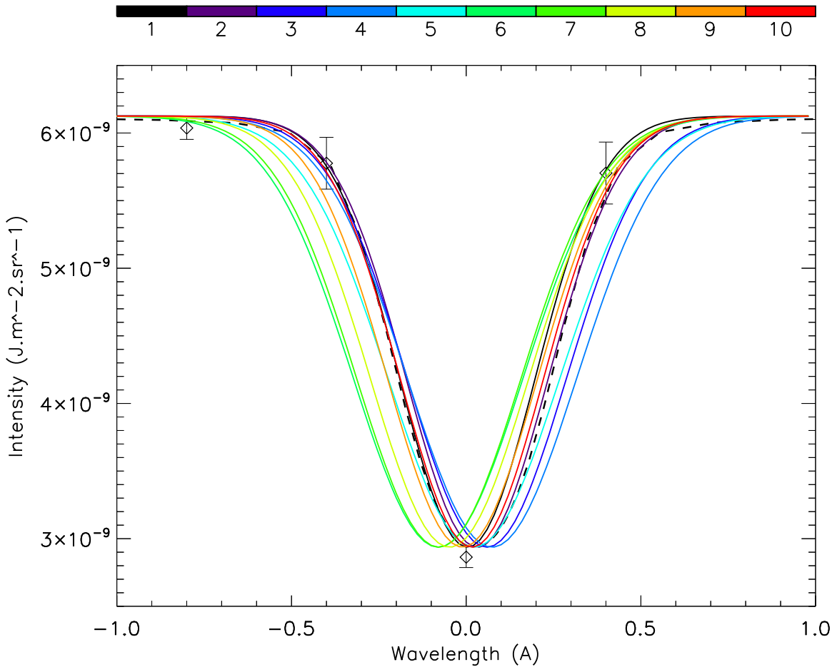
Figure 10. A series of interpolations of the H\alpha line profile in phase order based on the simulation result from the RH code as well as the relative intensities of the four H\alpha sub-bands. The dashed line represents the original emergent line profile (violet line in Figure 9 left panel), while each colored line represents Gaussian fitting to the four H\alpha line intensities at 10 times (marked with 10 vertical dashed lines in Figure 8). The color bar indicates the time bin. For these fits we kept the continuum and line-core intensities fixed and fit only line shift and line width. The error bars plotted for the first Gaussian fit were calculated based on the standard deviation of the light curves in the nearby quiet region for each of the four H\alpha sub-bands.
