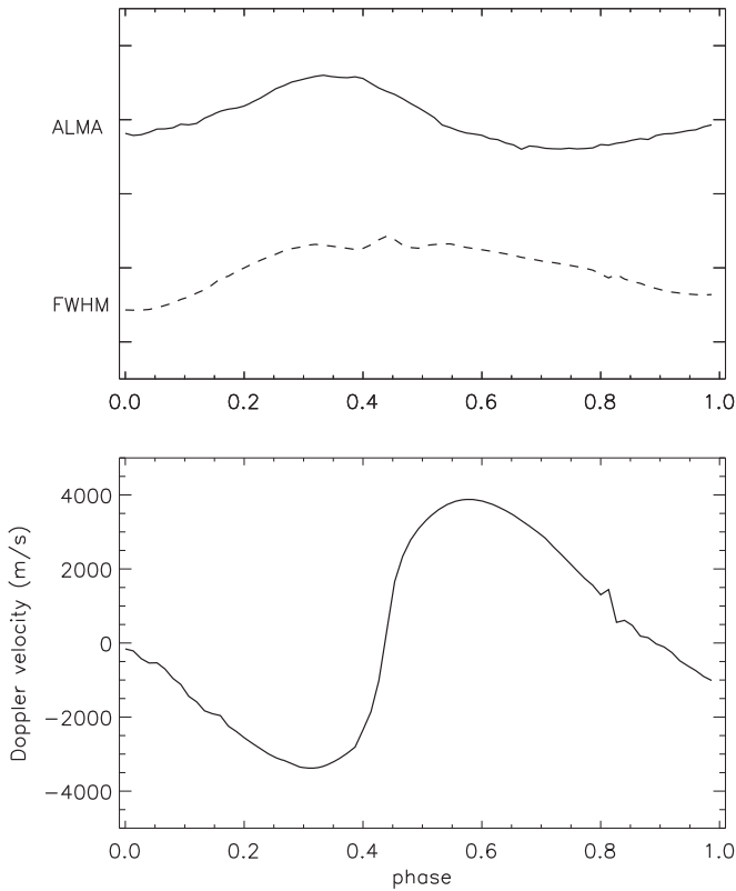
Figure 11. Top panel: a comparison between an ALMA light curve (first oscillation of t_2 ) and the FWHM of the Gaussian fitting in Figure 10. Bottom panel: the Doppler velocity corresponding to the H\alpha centerline shift in Figure 10. The upward Doppler velocity is treated as positive in the figure.
