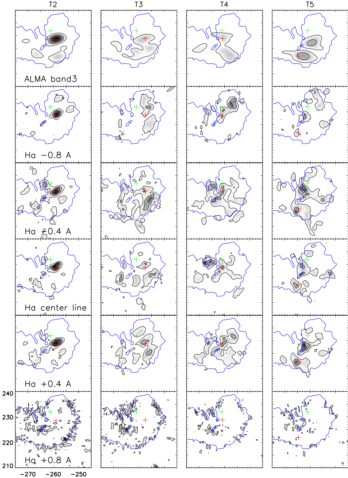
Figure 6. Spatial distribution and relative power level of 3 minute oscillations in various bands. For this comparison the H\alpha data have been temporally interpolated and spatially smoothed to match the ALMA resolution. The contours in ALMA and the H\alpha sub-band images represent 10%, 30%, 50%, 70% and 90% of the peak value of the 3 minute oscillation power in each wavelength. Red and green plus symbols mark regions of high and low power, respectively, whose light curves are plotted in Figure 7.
