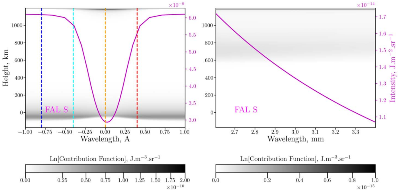
Figure 9. Spectral synthesis results obtained with the RH code. Left panel: intensity contribution function (gray shade) vs. height for the H\alpha line from the Fontenla, Avrett, & Loeser sunspot model (FAL S) that simulates a sunspot umbra, overlaid with the emergent line profile (violet line, scale on the right axis). The wavelengths are shown relative to the H\alpha line center, with four vertical dashed lines indicating the H\alpha sub-bands used for the study. The line colors follow the same scheme as in Figures 7 and 8. Right panel: contribution function for the emergent intensity for ALMA Band 3 wavelength range from the same FAL S model, overlaid with the emergent intensity profile (violet line).
