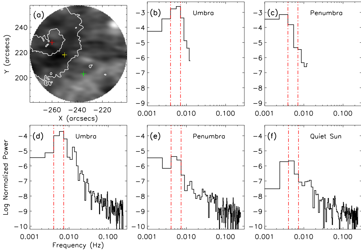
Figure 4. Three examples showing the power spectrum in the sunspot umbra, penumbra, and quiet Sun regions. (a) ALMA image for locating the sample points, marked with plus signs. The inner white contour is the boundary of the sunspot umbra while the outer contour is the boundary for the sunspot penumbra. (b) Power spectrum of GST H \alpha near blue wing ( -0.4 \text{ \AA} ) data from red point in the sunspot umbra showing a strong peak in the 3 minute oscillation band marked with dotted-dashed line. (c) The same as (b) for yellow point in the sunspot penumbra. (d) Power spectrum of ALMA data from the red point in the sunspot umbra. (e) (f) the same as (d) for sunspot penumbra and quiet Sun region.
