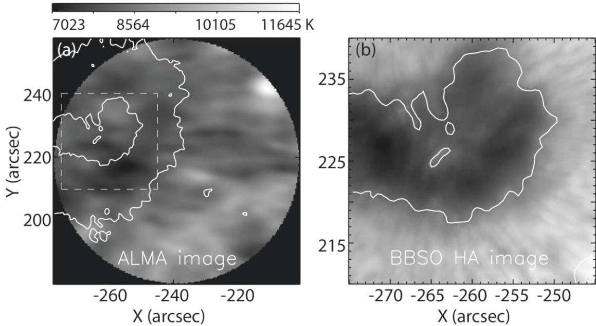
Figure 1. (a) ALMA brightness temperature image with contours from HMI continuum image showing the umbral and penumbral boundary of sunspot AR 12470 at 19:02 UT. The box marked with a dashed line shows the FOV of the BBSO GST H \alpha image in the right panel. (b) GST H \alpha near the blue wing ( -0.4 Å) image with the same HMI umbral contour.
