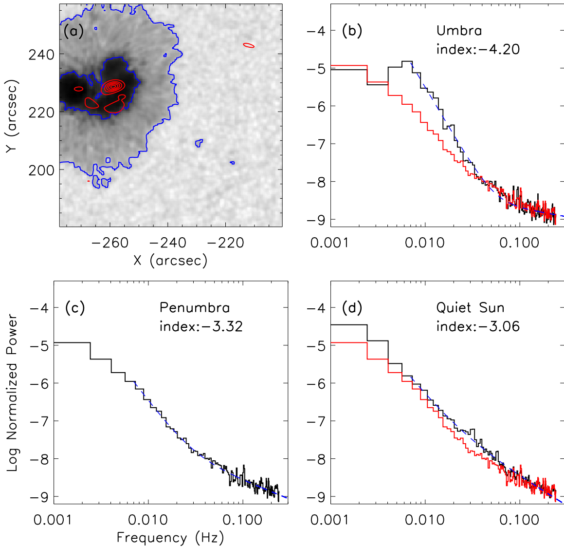
Figure 5. Comparison of ALMA power spectra averaged over umbral, penumbral, and quiet Sun regions. (a) HMI continuum image at 19:02 UT, overlaid with red contours showing the 3 minute oscillation power and blue contours outlining the umbra and penumbra from the HMI continuum image. (b) Averaged umbral power spectrum with blue dashed line showing a region well fit by a power law. (c) Same as (b) for the penumbral region. (d) the same as (b) for quiet Sun. The averaged penumbra power spectrum in panel (c) is over-plotted in red in both (b) and (d).
