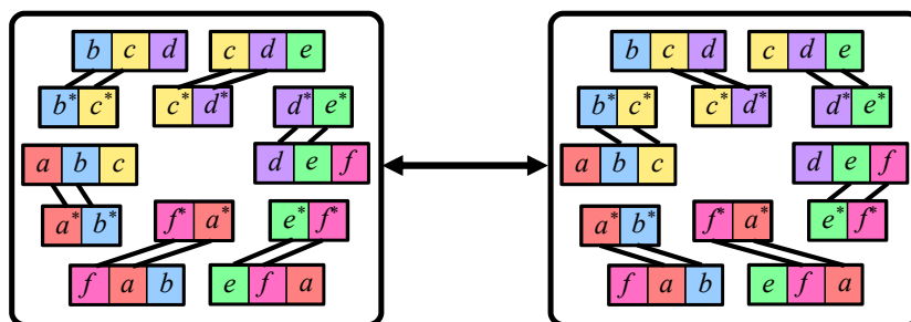
Figure 3 The two stable configurations of a variant of the circular translator cascade described in [2]. In the left configuration, the unstarred monomers are bound to their “left-side” companions (e.g. \{a, b, c\} is bound to \{a^*, b^*\} ), and in the right configuration, the unstarred monomers are bound to their “right-side” companions (e.g. \{a, b, c\} is bound to \{b^*, c^*\} ).
