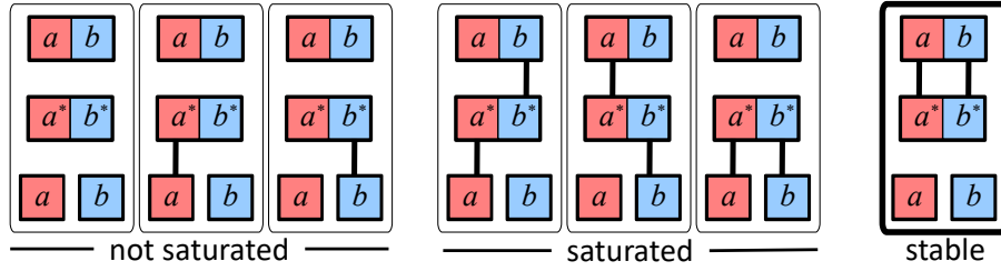
Figure 1 Example of a simple thermodynamic binding network (TBN). There are four monomers: \mathbf{m}_1 = \{a^*, b^*\} , \mathbf{m}_2 = \{a, b\} , \mathbf{m}_3 = \{a\} , \mathbf{m}_4 = \{b\} , with seven configurations shown: four of these configurations are saturated because they have the maximum of 2 bonds. Of these, three have 2 polymers and one has 3 polymers, making the latter the only stable configuration. Despite the suggestive lines between binding sites, the model of this paper ignores individual bonds, defining a configuration solely by how it partitions the set of monomers into polymers, assuming that a maximum number of bonds will form within each polymer. (Thus other configurations exist besides those shown, which would merge polymers shown without allowing new bonds to form.)
