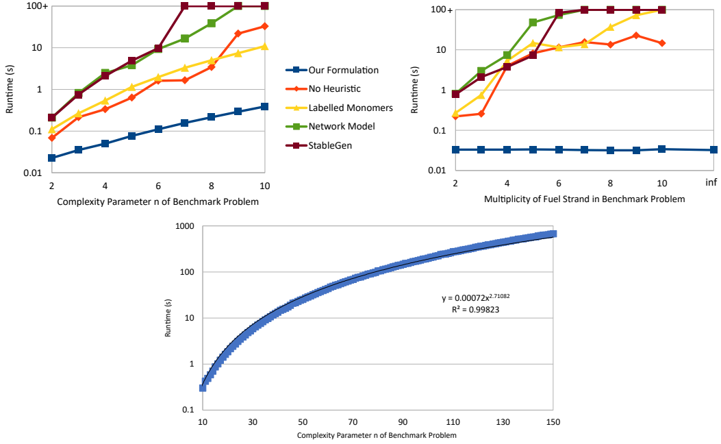
Figure 2 Empirical tests solving STABLECONFIGS for our benchmark problem based upon its complexity parameter n (left and bottom), and the multiplicity of the unstarred “fuel” strands (right). Our formulation is tested against several variations on the approach (which are described in the text) and the StableGen algorithm from [3]. The TBN is parameterized by n and contains the monomers G_n = \{x_{ij}^* : 1 \leq i, j \leq n\} , H_i = \{x_{ij} : 1 \leq j \leq n\} for all 1 \leq i \leq n , and V_j = \{x_{ij} : 1 \leq i \leq n\} \cup \{x_{ij} : j \leq i \leq n\} for all 1 \leq j \leq n . See Fig. 6 from [2] for a detailed explanation of this TBN and its operation. The vertical axis is log scale. Points at the top of the scale timed out after 100 seconds. The alternate formulations cannot solve the instance in the case of infinite fuel strands.
