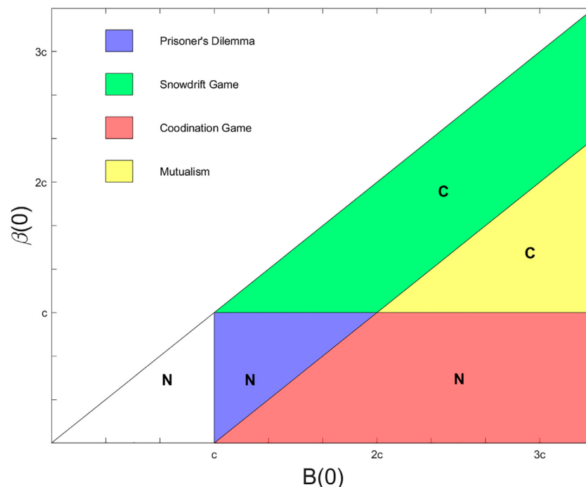
FIGURE 1 | Beyond the Prisoner's Dilemma. For different values of B(0) and \beta(0) , our evolutionary game theoretical model encompasses four regimes of classical games: Prisoner's Dilemma (blue), Snowdrift (green), Coordination (red), and mutualism (yellow). The regions are marked if we expect a communicative invasion of a non-communicative population to take over (C) or fail (N) with all-to-all connectivity. Results from Tripp et al. (2020).
