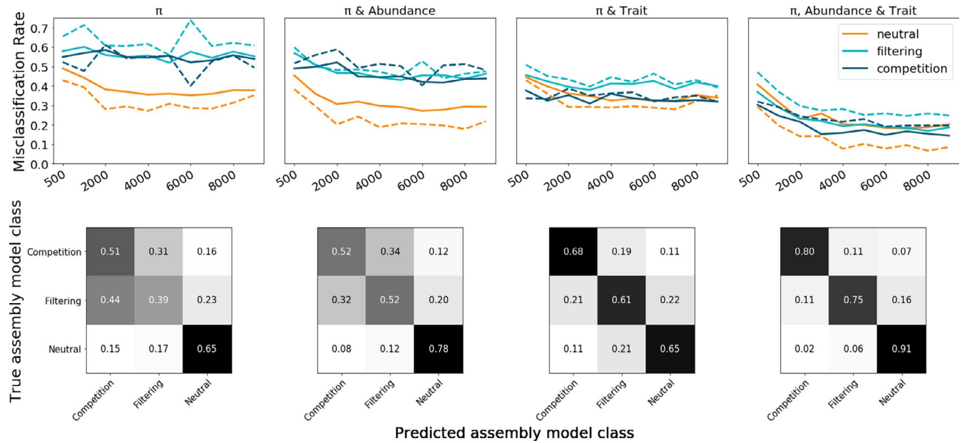
FIGURE 5 Machine learning classification error rates and confusion matrices. The top row shows random-forest misclassification error rates given different combinations of available data axes for varying sizes of local communities ( J ). Data axes used for each suite of simulations are indicated along the top of the figure. The x-axis indicates increasing sizes of J , from 500–10,000 in regular intervals. The y-axis indicates probability of assembly model misclassification, averaged over 1000 simulations per model class for each J (i.e., lower values indicate more accurate classification). In the figure, orange shows neutral simulations, aqua shows filtering, and dark blue shows competition. Solid lines indicate 1 - precision and dashed lines indicate 1 - recall. The bottom row shows confusion matrices depicting detailed model misclassification rates for data availability scenarios given J values between 9000 and 10,000. In these figures, values on the diagonals indicate the proportion of accurately classified simulations for each model class. Off-diagonal values indicate misclassified simulations
