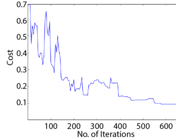
Fig. 7: The plot of our optimization process for the result of Fig. 5
