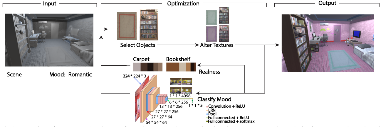
Fig. 2: An overview of our approach. The user first selects a mood type and a virtual room as input. The optimization process then takes place - objects in the scene are selected so their textures can be altered. Images are taken to capture the outlook of the current scene, based on which the current mood cost is calculated using a CNN classifier. A realness cost is also computed to determine how realistic the textures are. The optimization process proceeds iteratively. The output is the scene optimized with respect to the target mood.
