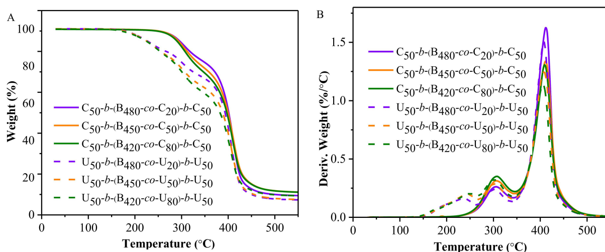
Figure 2. (A) TGA thermogram curves and (B) the corresponding weight derivative curves of CyA and UCyA triblock copolymers with varied amounts of hydrogen bonding unit.
