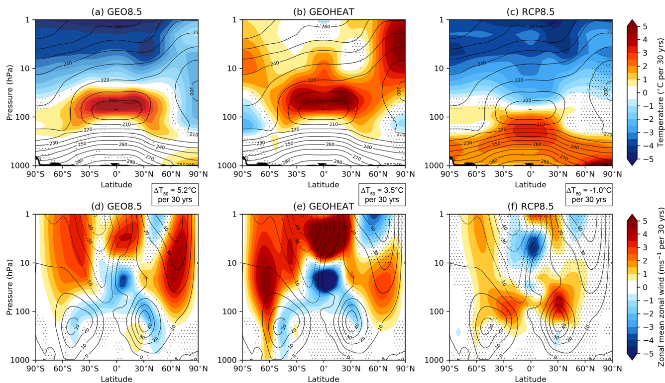
Figure 3. Trends in DJF zonal mean temperature and zonal winds. Shown are ensemble mean linear trends in temperature (a–c; shading; degrees Celsius per 30 years) and zonal wind (d–f; shading; meters per second per 30 years). Responses are shown for (a, d) GEO8.5, (b, e) GEOHEAT and (c, f) RCP8.5. Contours show the Base climatology (2010–2030). Stippling indicates trends that are not statistically significant at the 95 % confidence level under a one sample, two-sided Student's t test using the standard deviation across ensemble members. \Delta T_{50} values for each experiment give the ensemble mean and tropical average temperature trend (30° S–30° N) minus the NH polar cap average trend (60–90° N) at 50 hPa.
