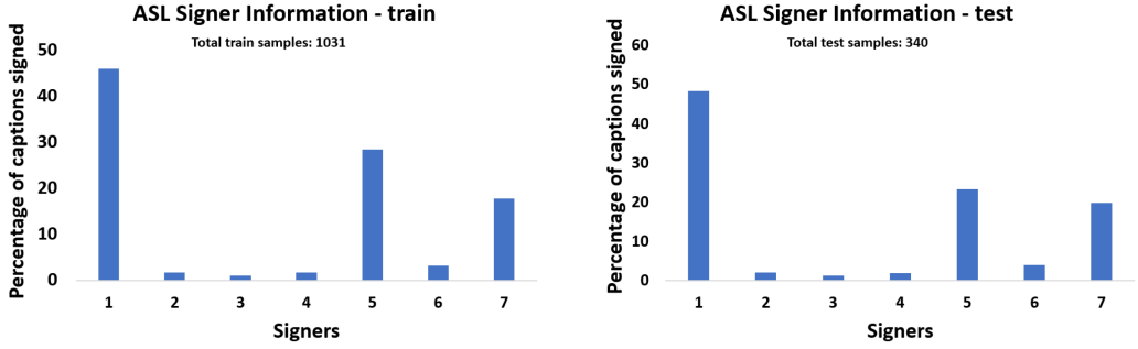
Fig. 9. Graph representing number of signs annotated by each signer in the ASL dataset.
