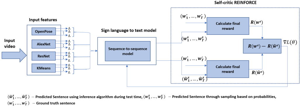
Fig. 4. Sign language to text model using reinforcement learning.
