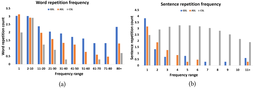
Fig. 6. (a) Word repetition frequency for unique utterances. (b) Sentence repetition frequency. The Y axis represents the log10 scale.
