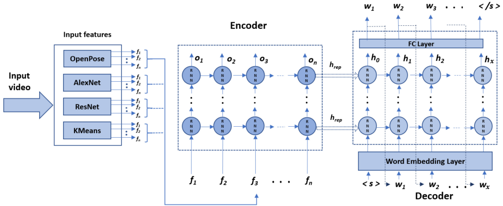
Fig. 1. Sequence-to-sequence model without attention.
