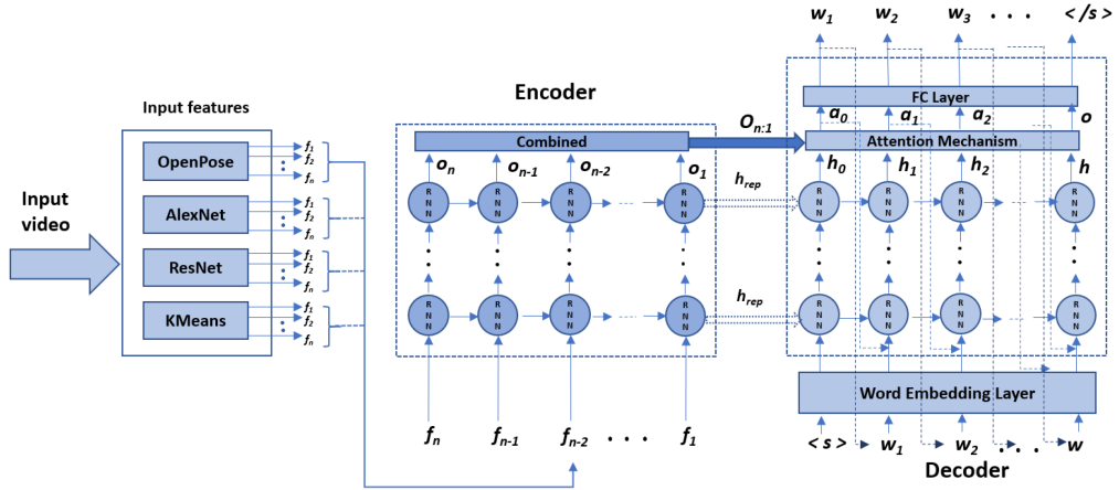
Fig. 2. Sequence-to-sequence model with attention mechanism.
