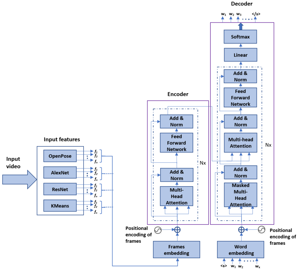
Fig. 3. The baseline transformer model.
