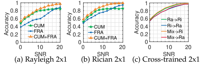
Fig. 16: Accuracy with increasing SNR over a Rayleigh (a) and Rician (b) channel with 2x1 sensing. SYMMeTRY with the combined CUM+FRA features outperforms counterparts across all SNR regimes in both channel conditions. (c) Accuracy of the CUM+FRA feature with cross-channel training. SYMMeTRY 's performance remains high and consistent with the same-channel training.
