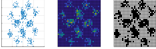
Fig. 7: Converting IQ samples to a binary matrix for box-counting.
