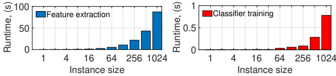
Fig. 23: SYMMeTRY runtime for feature extraction (left) and classifier training (right) with exponentially-increasing instance size. Both feature extraction and training time grow linearly with the instance size.
