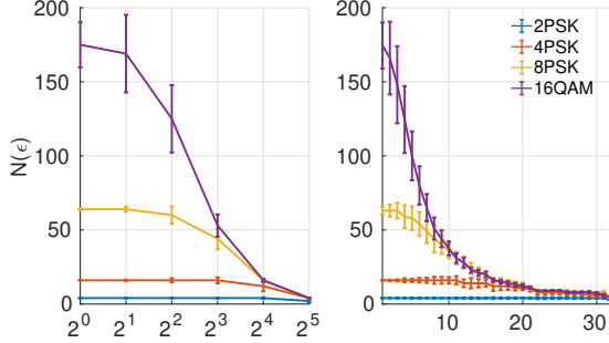
Fig. 8: An illustrative comparison of the fractal feature vectors for four modulations in 2-transmitter MIMO using exponential (left) and linear (right) resolution schedules T . X-axis is the box size \epsilon .
