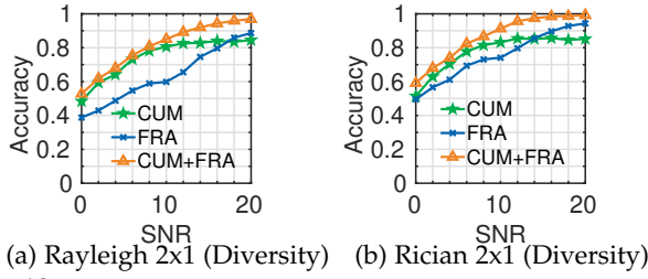
(a) Rayleigh 2x1 (Diversity) (b) Rician 2x1 (Diversity) Fig. 18: Accuracy with increasing SNR over a Rayleigh (a) and Rician (b) channel with 2x1 sensing. The MIMO transmitter uses spatial diversity coding with Alamouti's code. SYMMeTRY with the combined CUM+FRA features outperforms counterparts across all SNR regimes in both channel conditions. The performance is similar to that of MIMO with spatial multiplexing (Fig. 16).
