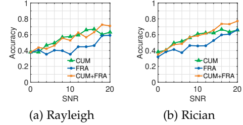
(a) Rayleigh (b) Rician Fig. 20: Accuracy with increasing SNR over a Rayleigh (a) and Rician (b) channel for high-order modulations (32/64/128QAM).
