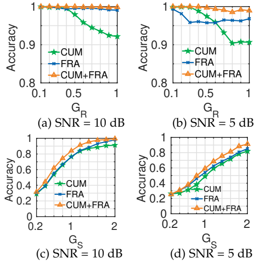
Fig. 15: Effects of constellation geometry as controlled by the channel gain ratio G_R (controlling symbol overlap) and the channel gain sum G_S (controlling symbol spread) in time-variant channels. (a), (b) show accuracy as a function of G_R for mid- and low-SNR. (c), (d) show accuracy as a function of G_S for mid- and low-SNR. FRA+CUM outperforms counterparts across all settings.
