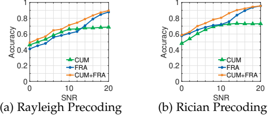
(a) Rayleigh Precoding (b) Rician Precoding Fig. 19: Accuracy for MIMO with precoding with increasing SNR over a Rayleigh (a) and Rician (b) channel with 2x1 sensing. We explore three realizations of a 2x2 MIMO transmitter with precoding: BPSK+QPSK, QPSK+8PSK and 8PSK+16QAM. SYMMeTRY with the combined CUM+FRA features outperforms counterparts across all SNR regimes in both channel conditions.
