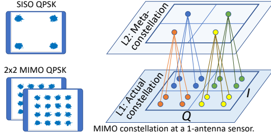
Fig. 1: Illustration of MIMO self-similarity for 2x2 QPSK MIMO.
