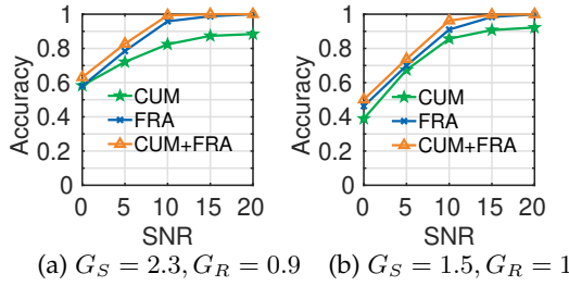
Fig. 12: Accuracy with varying SNR for two channels H1 (a) and H2 (b). The channel gain sum G_S for H1 is larger than that for H2 (i.e. constellations from H1 are spread out and easier to detect than H2 ). FRA and FRA+CUM outperform CUM across all SNR regimes. High-gain channels ( H1 ), further emphasize the advantage of FRA and CUM+FRA over classical CUM.
