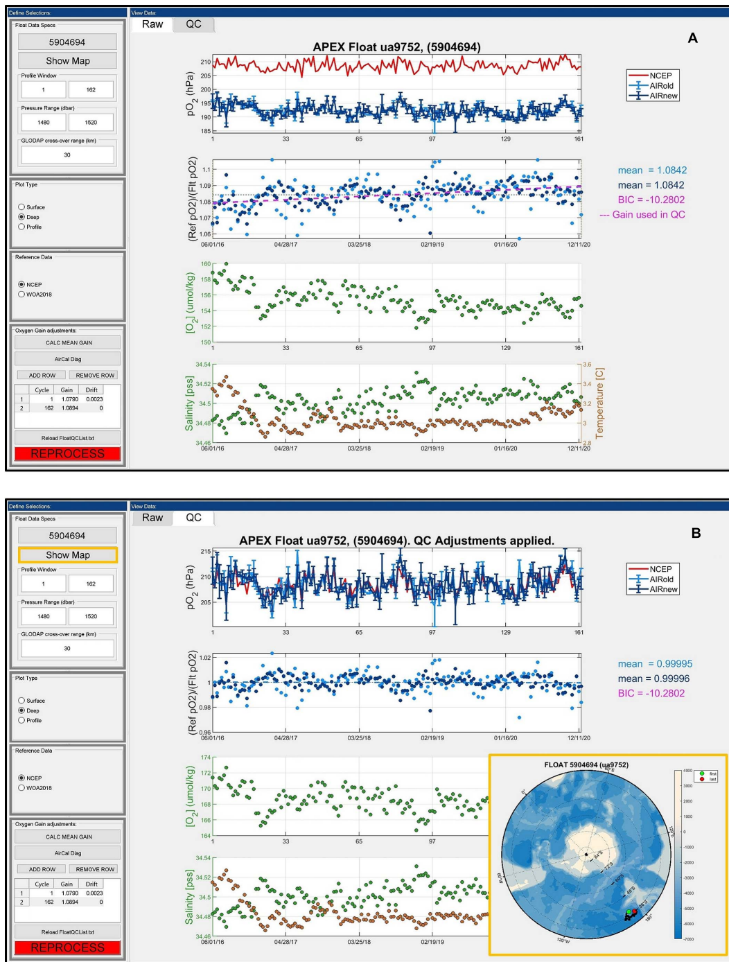
FIGURE 3 | SAGE- O_2 software interface showing results of the calibration for sample float 9752, WMO 5904694. The view in (A) displays the raw oxygen float data against the reference, while the view in (B) displays float data that was adjusted using the coefficients derived through the software. The map display functionality is also indicated in (B) .
