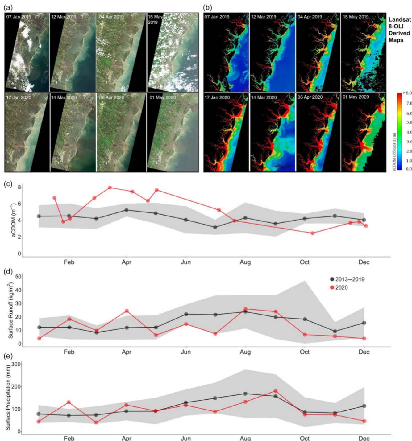
FIGURE 6 Comparison of (a) monthly true color images and (b) estimates of absorption by colored dissolved organic matter (CDOM [ a_{CDOM} ]) at 355 nm ( m^{-1} ) in Georgia coastal waters in 2019 and 2020. Time series of (c) Landsat 8 derived a CDOM for the Georgia Coastal Ecosystems Long Term Ecological Research (LTER) domain showing monthly means for the years 2013–2019 compared to 2020. Time series of (d) area-averaged monthly means (2013–2019) of surface runoff compared to 2020 and (e) monthly means of surface precipitation (2013–2019) compared to 2020 for coastal Georgia. The surface runoff and precipitation data were derived from NASA's MERRA-2 long-term global re-analysis database (MERRA-2 Model M2TMNXLND v5.12.4). Data for 2013–2019 are represented as means (black points) and SDs (gray shaded region), and 2020 data are represented as red points. Source: Landsat 8-OLI. The CDOM model ( R^2 = 0.74 ) used in this study was originally developed for Landsat 5-TM (Joshi & D'Sa, 2015). However, both Landsat 8-OLI and Landsat 5-TM have similar green and red bands (band centers and bandwidths) that were used in the CDOM model, and therefore, we assume the impact of the sensor differences would be minimal in CDOM estimation. Note about uncertainty: The model was developed for Barataria Bay, Louisiana. We have not tuned the model for coastal Georgia because of the lack of in situ data
