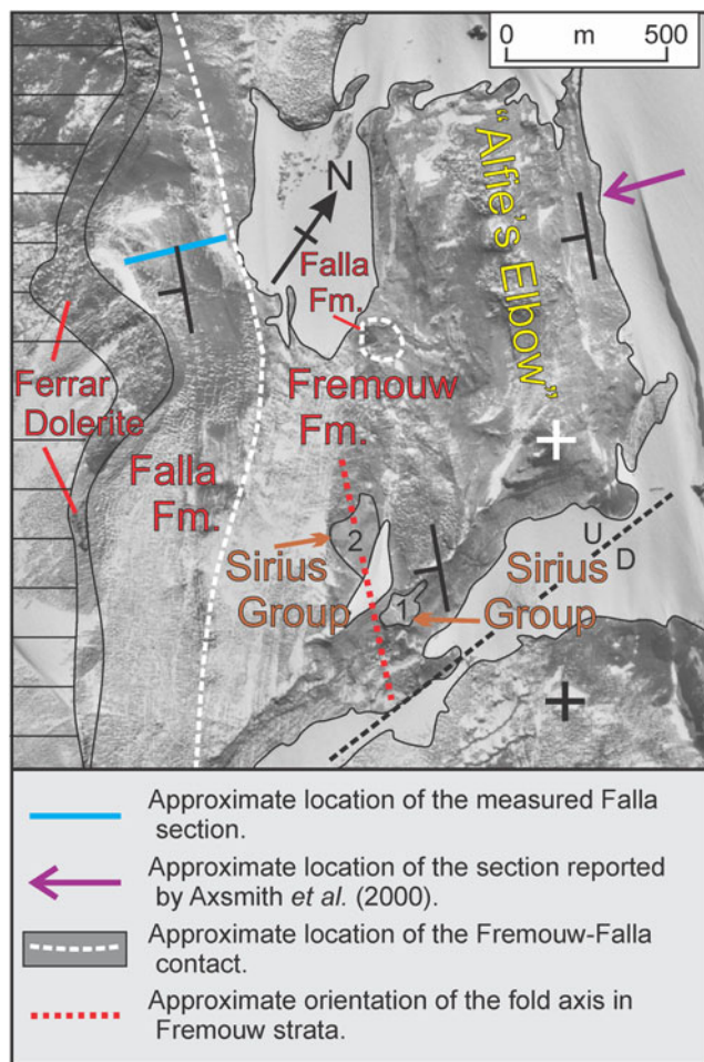
Fig. 5. Geological sketch map of the 'Alfie's Elbow' region of Schroeder Hill. A small remnant of basal Falla beds, in the form of quartz-pebble conglomerate, is inferred on the Fremouw dip slope south-west of 'Alfie's Elbow' and is indicated by the enclosed dashed white line. The heavy dashed black line indicates the location of the inferred fault juxtaposing the Fremouw and Falla beds. The horizontal line pattern to the left of the Ferrar Dolerite sill denotes dolerite overlain by surficial debris. Attitude symbols indicate low dips to the south-south-west. Enlarged from Polar Geospatial Center/USGS aerial photo TMA 788 033 F32(V).
