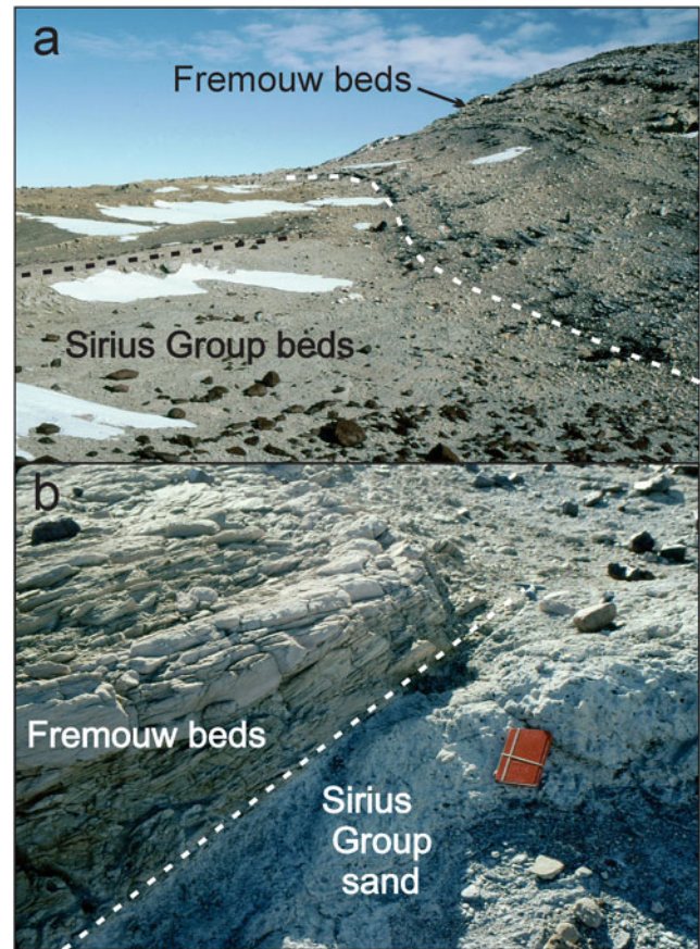
Fig. 8. a. Closer view of gently folded Fremouw beds in contact with Sirius strata. The white dashed line marks the contact. The black dashed line marks bedding in Sirius strata. The direction of the view is indicated in Fig. 7a. b. Pale-coloured Sirius Group sand wedged under dipping Fremouw strata located at the south-east edge. This is the south-east edge of Sirius Site 1 in Fig. 5. The direction of view is indicated on Fig. 7b.
