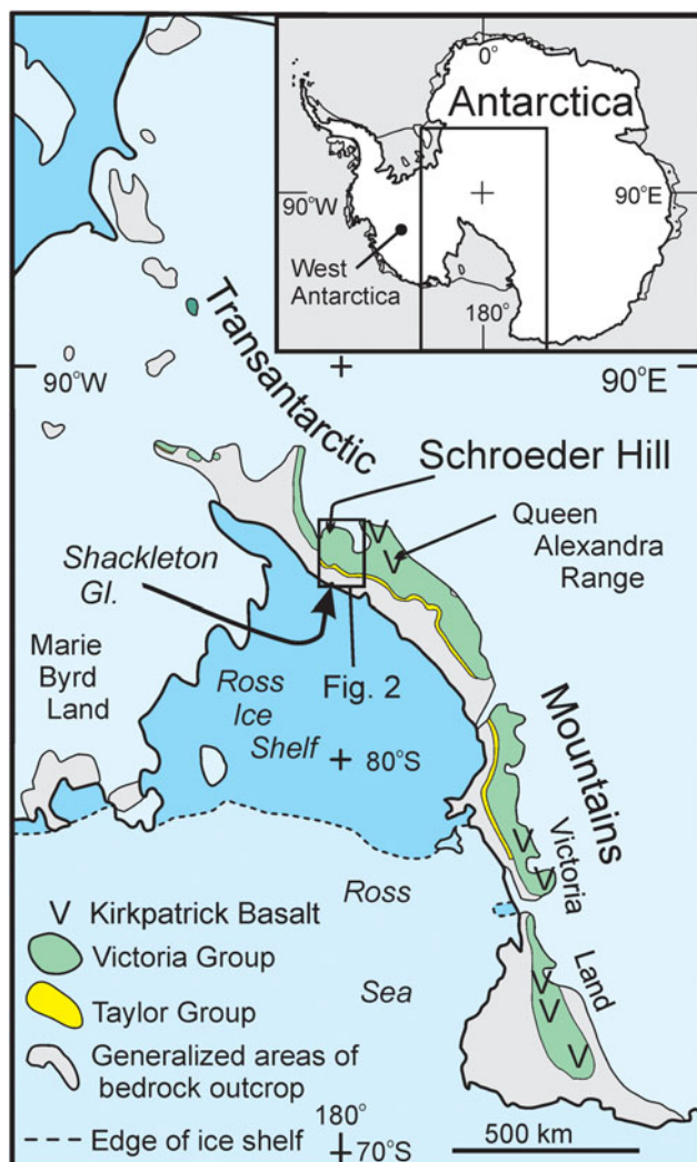
Fig. 1. Location of Schroeder Hill, central Transantarctic Mountains, Antarctica.
