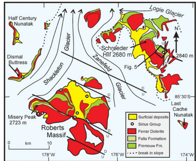
Fig. 4. Geological sketch map of the upper Shackleton Glacier region. Sirius Group localities at Half Century Nunatak, Dismal Buttress and Roberts Massif are from Hambrey et al. (2003). Extensive dolerite surfaces at Roberts Massif, at Schroeder Hill and to the south-east have a veneer of surficial debris. 'Alfie's Elbow' is located within the box outlining Fig. 5.
