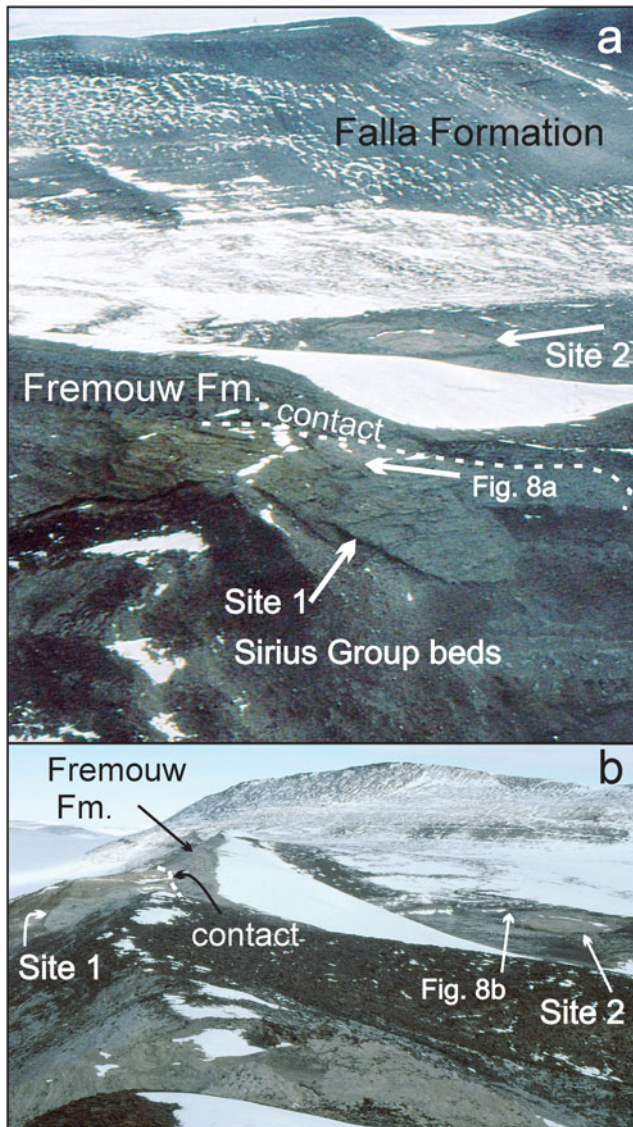
Fig. 7. a. Photograph showing the locations of the two Sirius deposits (see also Fig. 5). View towards the west approximately from the position of the black cross in Fig. 5. b. View towards the south-east from the point marked by a white cross in Fig. 5 of the same two Sirius sediment localities.
