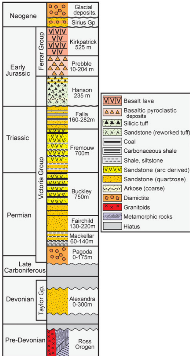
Fig. 3. Simplified stratigraphic column for the central Transantarctic Mountains (Queen Alexandra Range to the Shackleton Glacier region).
