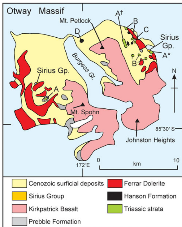
Fig. 9. Location map for Otway Massif. Site A: Fremouw Formation megaclasts; Site A*: location of the Fremouw Formation section illustrated in Fig. 6; site A†: see text; sites labelled B: Falla Formation megaclasts; Site C: possible Hanson Formation outcrop; Site D: Hanson Formation strata. Map modified from Elliot & Hanson (2001).
