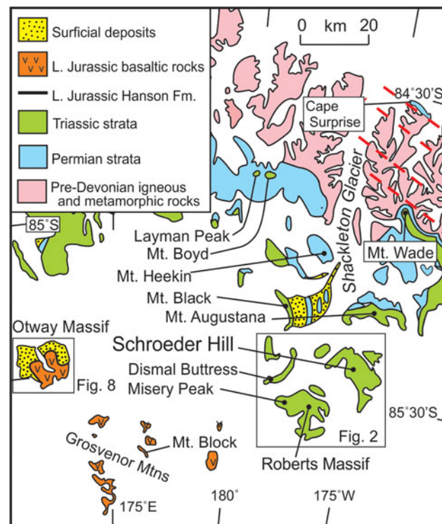
Fig. 2. Geological sketch map of the Shackleton Glacier region. Dashed red lines between Mount Wade and Cape Surprise are the interpreted positions of major faults (Miller et al. 2010).
