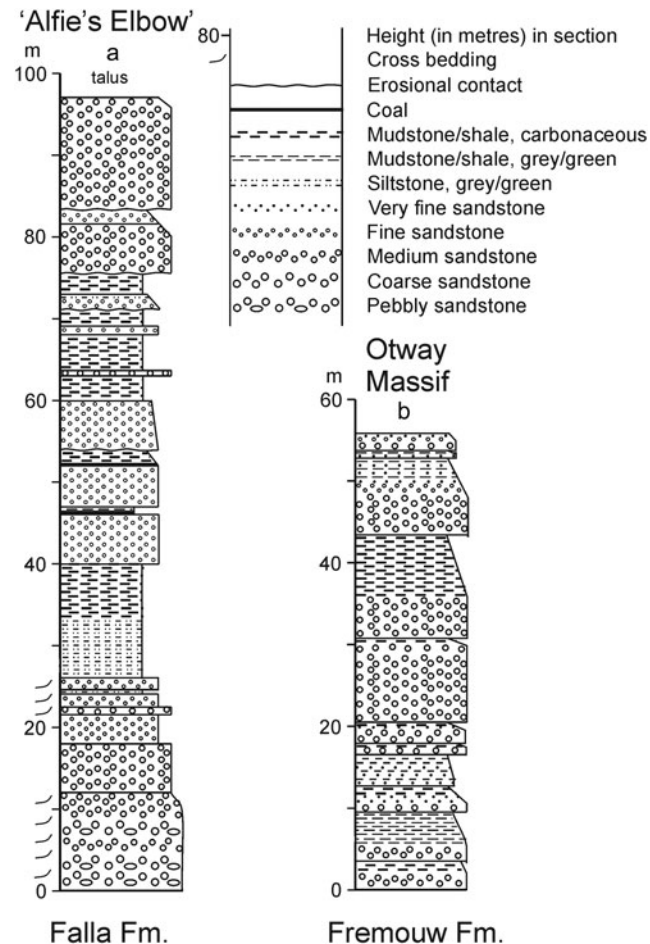
Fig. 6. a. Stratigraphic column for Falla beds south-west of 'Alfie's Elbow' (location in Fig. 5). b. Stratigraphic column for Fremouw beds at Otway Massif (location A* in Fig. 9). Fremouw sandstones are volcanoclastic; Falla sandstones are quartzose.
