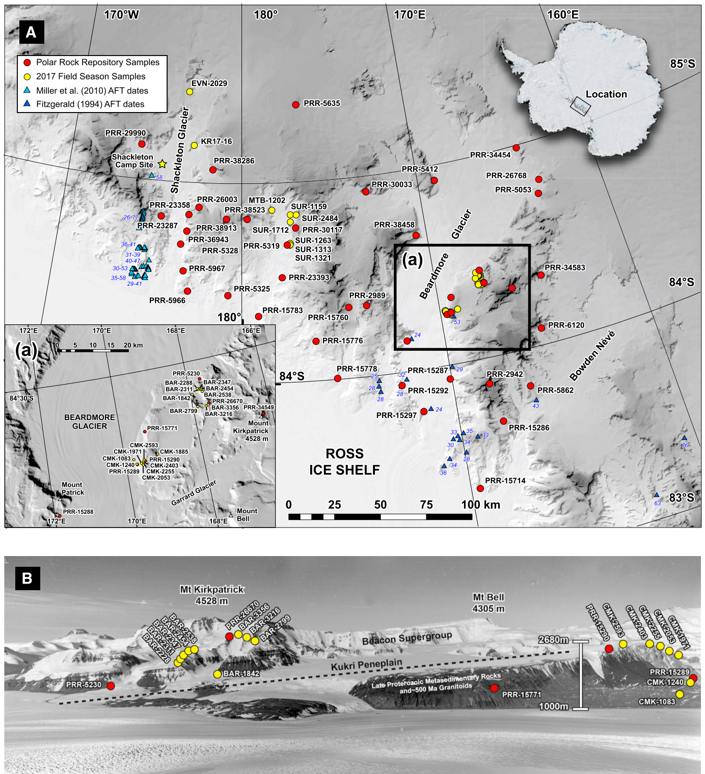
Fig. 2. Sample Locations. (a) Map of samples from the field (CMK- Cloudmaker; BAR – Barnes Peak; KR-Kitching Ridge; EVN- Everett Nunatak; MTB- Mt. Bellows) and from the Polar Rock Repository (PRR), and previous thermochronology studies; (b) annotated photograph (cropped and edited for clarity) showing the relative locations of vertical transect samples relative to the tilt of the Kukri Peneplain and Beacon supergroup strata. Restoring the dip of the unconformity to horizontal would add ~0.5 km of additional vertical offset between the two transects (assuming regional tilting was associated with post-exhumation rift-flank uplift). Aerial photograph (CA03950312) and DEM courtesy of the Polar Geospatial Center.
