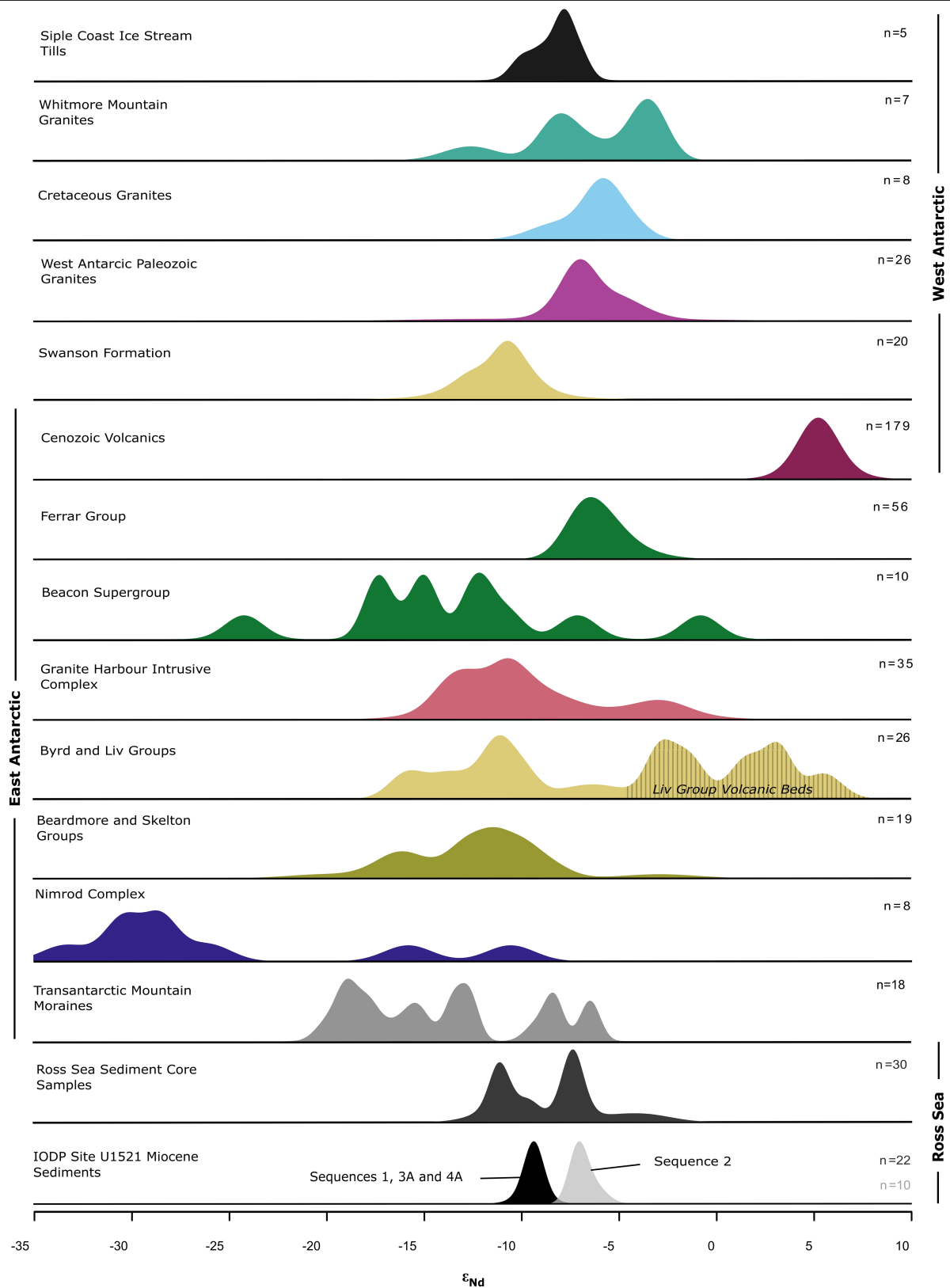
Extended Data Fig. 5 | Kernel density estimate plots for literature measurements of rock \epsilon_{Nd} compared to measurements on fine-grained Miocene detritus from Site U1521. For references and a list of all the data, see
