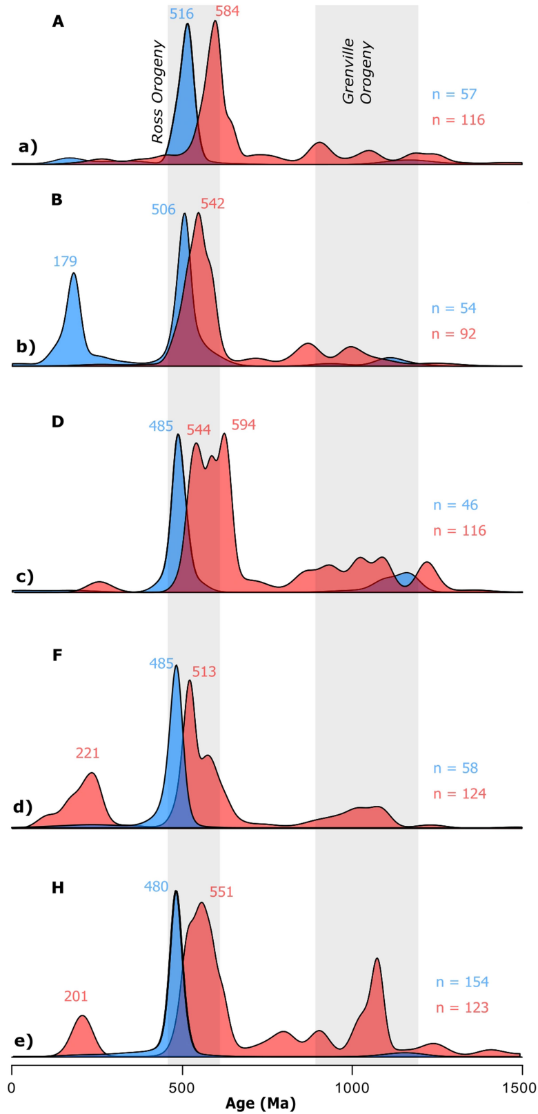
Extended Data Fig. 6 | Kernel density estimates for hornblende ^{40}\text{Ar}/^{39}\text{Ar} ages compared to zircon U-Pb ages younger than 1500 Ma. The two dating methods are shown in red and blue, respectively. Bold letters correspond with
