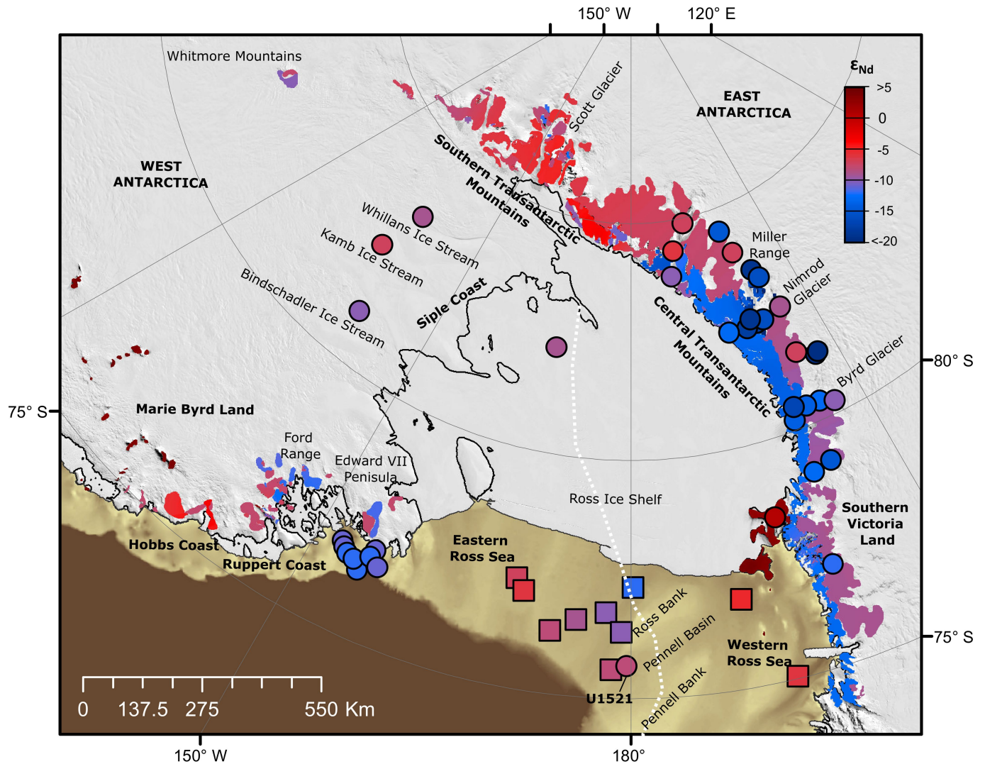
Extended Data Fig. 4 | Map of approximate \epsilon_{Nd} values in rocks and offshore sediments from around the Ross Sea embayment. Epsilon Nd values are overlain on MODIS imagery 200 and the BedMachine Antarctica V1 modern bed topography 43,44 , with the MEaSUREs grounding line and ice sheet margin shown 45,46 . The approximate boundary between West and East Antarctic lithosphere is shown using a white dashed line 47 . Modern/late Holocene and terrestrial till samples are represented by circles with the same colour bar 28,30,55 . Although ice flow patterns have changed since their deposition, Last Glacial
