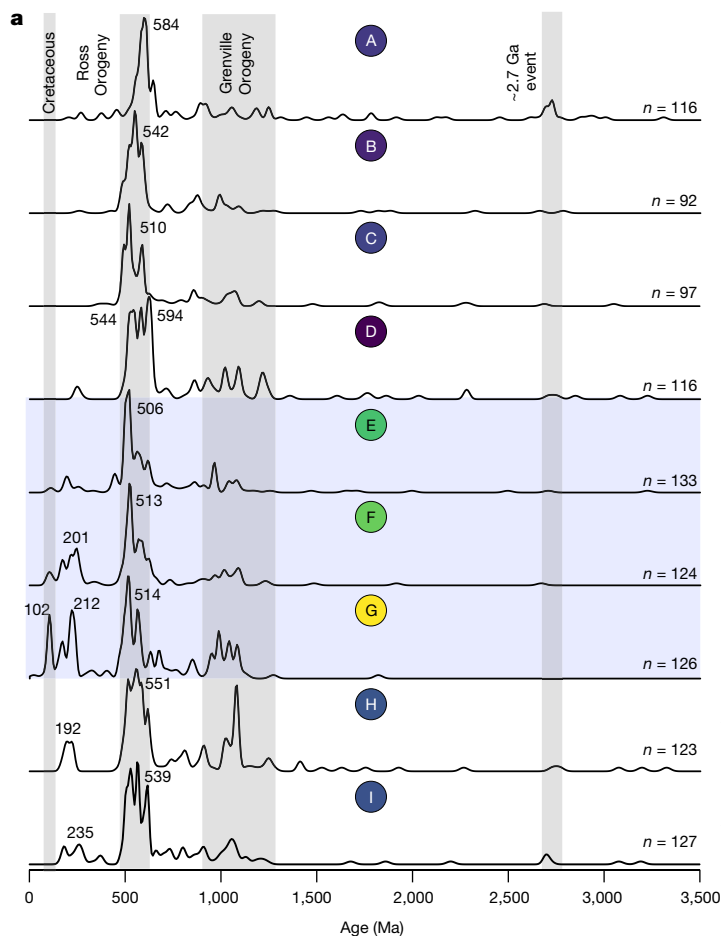
Fig. 3 | Site U1521 detrital zircon U–Pb age distributions. a , Data displayed as kernel density estimates (KDEs). When present, large Ross Orogeny (~600–500 Ma), Triassic (~240–190 Ma) and Cretaceous (~100 Ma) age peaks are labelled. The age ranges of the Ross Orogeny, Grenville Orogeny and an ~2.7 Ga event recorded in Ross Sea sedimentary strata are illustrated using grey-shaded bars. The sub-bottom depth midpoints of the samples are shown in Fig. 2 and listed in the Methods section. b , Same data as in (a), displayed as a multidimensional scaling (MDS) map calculated using the Kolmogorov–Smirnov statistic 51 . Stress (a measurement of the goodness of fit between the disparities and the fitted distances 51 ) = 0.072. An MDS plot visualizes the degree of similarity between samples, with the proximity of sample points
