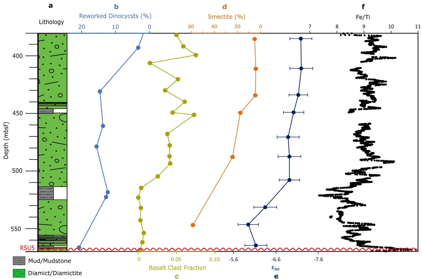
Extended Data Fig. 7 | Close up of the Site U1521 interval with a West Antarctic provenance. The stratigraphic log (a) is displayed alongside the percentage of reworked dinocysts (b), basalt clast fraction (c), relative
