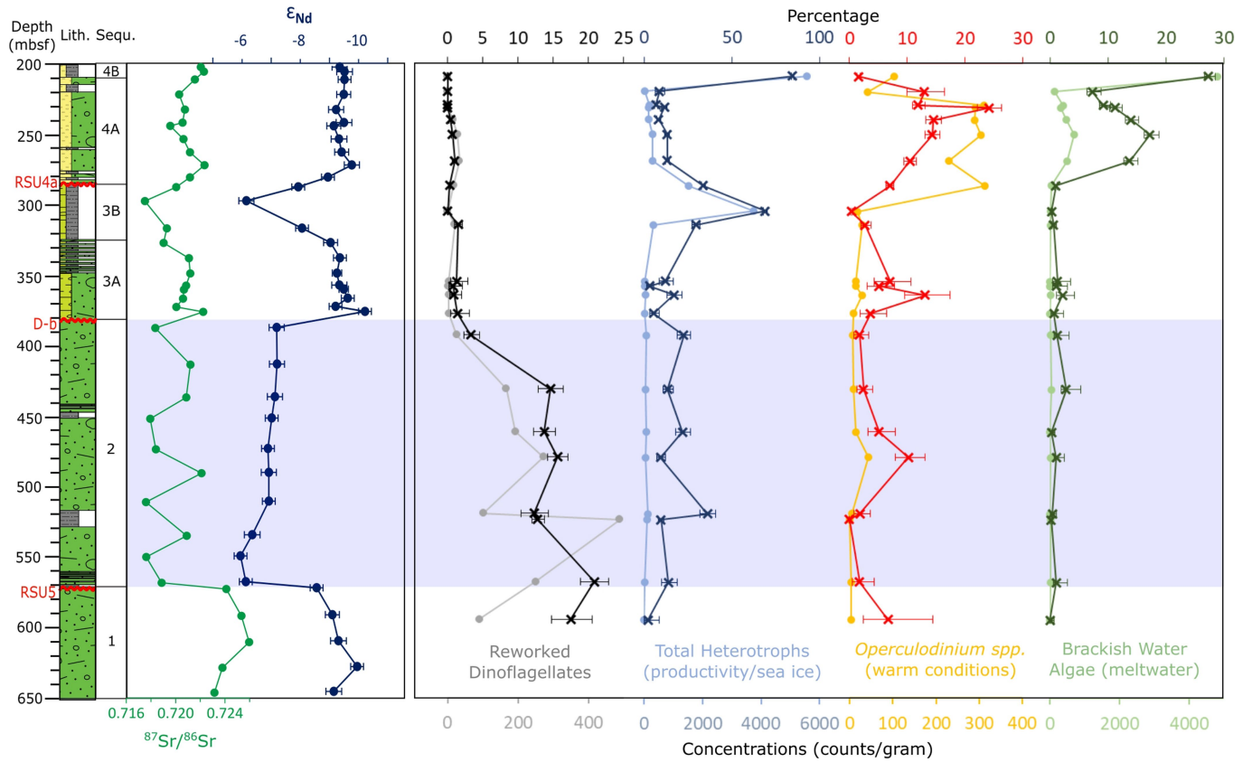
Extended Data Fig. 2 | Selected palynological counts compared to strontium and neodymium isotope data. Palynological data are reported as percentages (crosses) and counts/gram (circles). The blue shaded area
