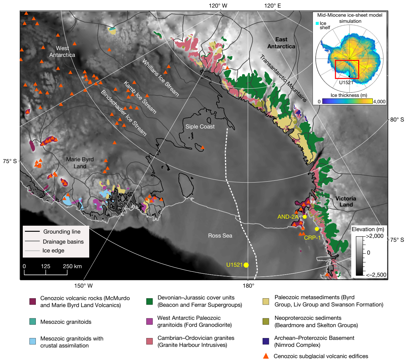
Fig. 1 | Site U1521 location and surrounding geology. The outcropping regional geology around the Ross Sea 42 (© SCAR GeoMAP and GNS Science 2019) is overlain on the BedMachine Antarctica V1 modern bed topography 43,44 . The MEaSURES grounding line, ice-sheet margin and basins are used 45,46 and the map was produced using ArcGIS software. IODP Site U1521 is located on the outer continental shelf of the central Ross Sea. Locations referenced in the text are labelled, including the ANDRILL 2A (AND-2A) and Cape Roberts Project 1 (CRP-1) drill sites. The white dashed line indicates the boundary between East and West
