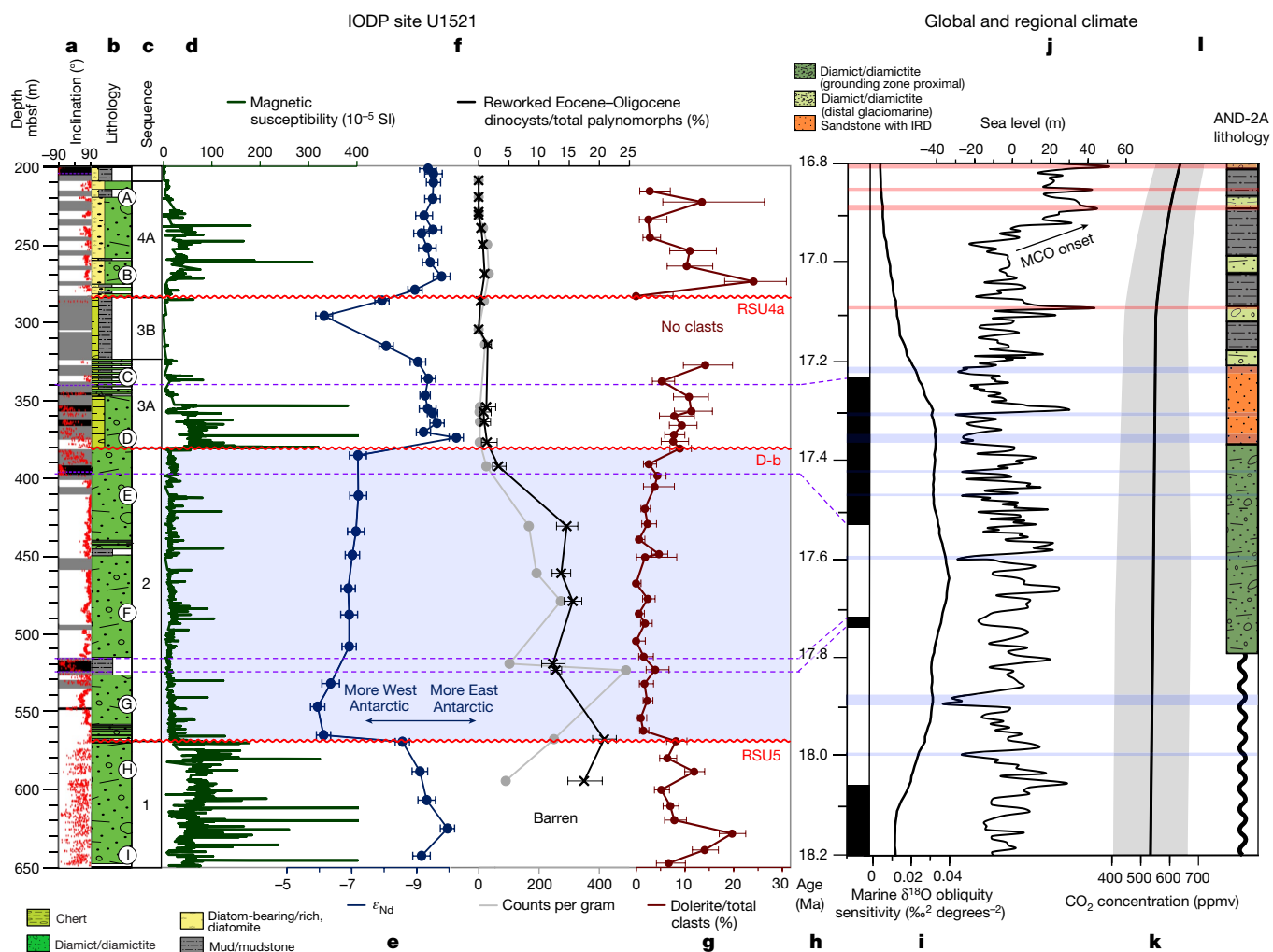
Fig. 2 | Selected provenance proxies from IODP Site U1521 compared with Early Miocene climate records. The light-blue-shaded section (Sequence 2) highlights the interval with sediments of predominantly West Antarctic provenance. The depth of Ross Sea Unconformity (RSU) 4a and 5 and seismic surface D-b are indicated in red 23 . a , Site U1521 inclination data after 20 mT demagnetization (red points) 26 and polarity interpretation (white = reverse polarity, black = normal polarity, grey = no interpretation). b , Site U1521 lithostratigraphy 26 . c , Chronostratigraphic sequences. The circled letters between (b) and (c) mark the depths of the zircon U-Pb samples (Fig. 3). d , Magnetic susceptibility measured on the whole core 26 . e , Neodymium isotope signature of the fine fraction. Error bars are 2 s.d. external reproducibility; for provenance interpretations, see Extended Data Fig. 4 and references in Supplementary Information. f , Abundance of Eocene–Oligocene dinocysts as a
