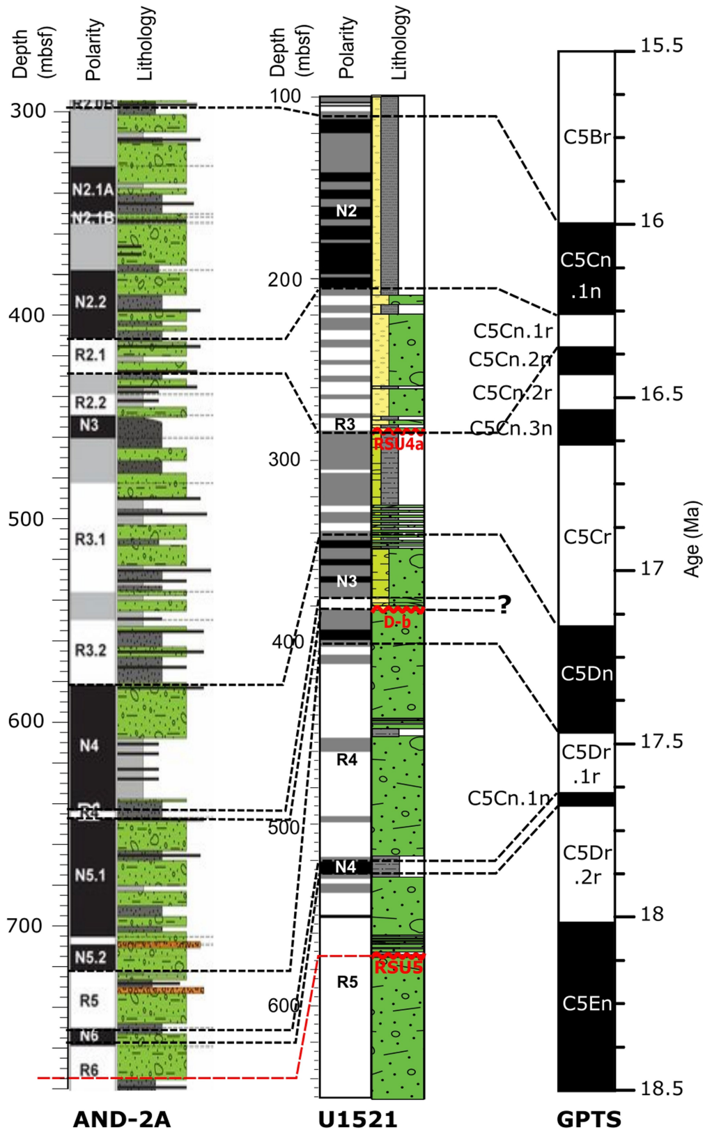
Extended Data Fig. 8 | Correlation of Site U1521 magnetostratigraphic tie points. Shown are correlations between the AND-2A record 11 , Site U1521 26 and the GPTS 49 .
