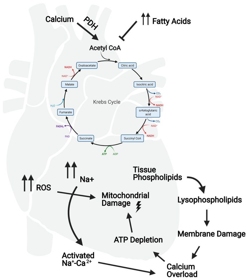
Figure 5. Mitochondrial dysfunction in ischemia. It is currently believed that irreversible ischemic damage is due to 1) loss of ATP, 2) supraphysiological free fatty acids levels, 3) formation of excess reactive oxygen species (ROS), 4) cellular calcium overload, and finally, 5) sodium pump inhibition. Figure created with BioRender.
