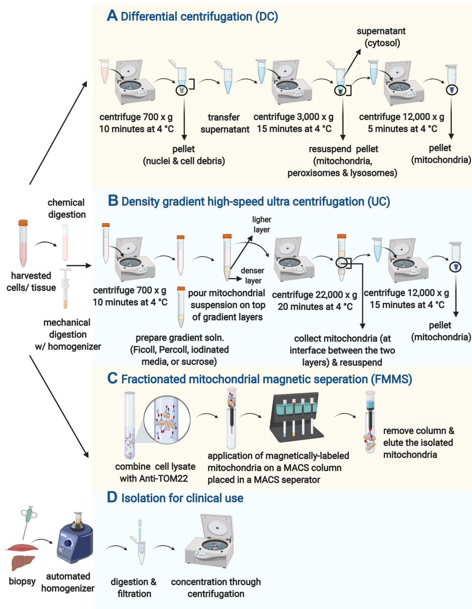
Figure 1. Mitochondrial isolation approaches in a glance. Current mitochondrial isolation techniques include A : differential centrifugation (DC). B : density gradient high-speed ultracentrifugation (UC). C : fractionated mitochondrial magnetic separation (FMMS). D : isolation for clinical use. Figure created with BioRender.
