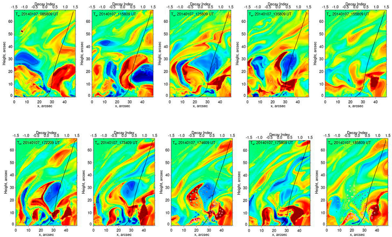
FIGURE 4 | Field line twist, T_W , maps shown for several instances for the west flux rope (FR). The T_W was calculated on a vertical plane orthogonal to the axis of an eruptive AR filament. The images are scaled between -2 < T_W < 2 , while contours outline areas with |T_W| > 1 . The black curve is the decay index profile calculated along the flaring PIL at x = 25'' . The x-axis begins at the top end of the cross-section ( Figure 1 ) and the sunspot is outside the FOV on the left side of the panels. The y-axis represents the height above the photosphere. The color coded dots in 17:46:09 and 18:58:09 UT panels indicate the locations through which we traced the fields lines shown in Figure 5 .
