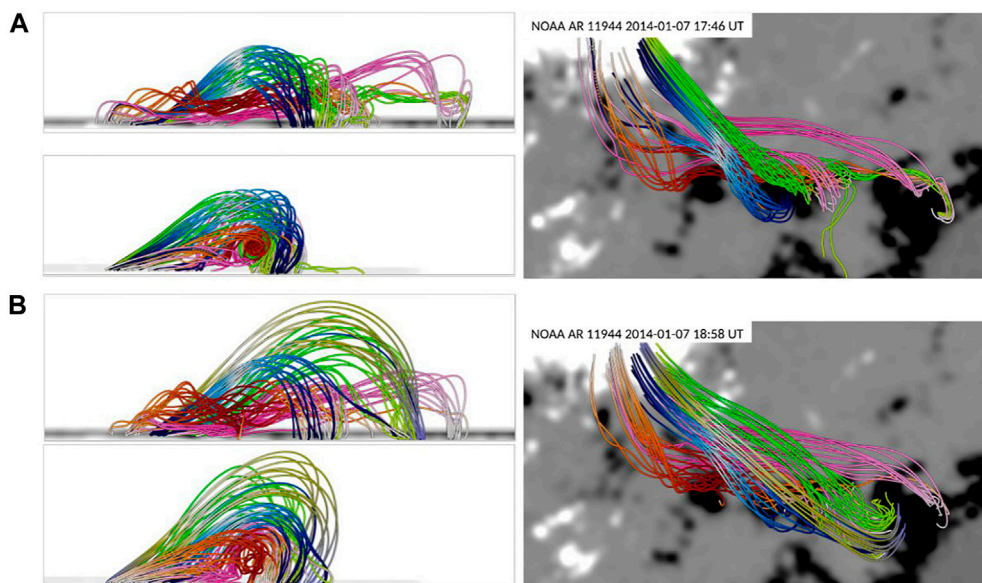
FIGURE 5 | Results of magnetic field extrapolation using a pre-flare 17:46 UT, (A) and post-flare 18:58 UT, (B) magnetic field measurements. The FOV shown is 140 \times 70 \times 70'' and is located at 55 < x < 220 and -180 < y < -80 in Figure 1 . Colored lines highlight various magnetic flux systems associated with the twist structures shown in Figure 4 .
