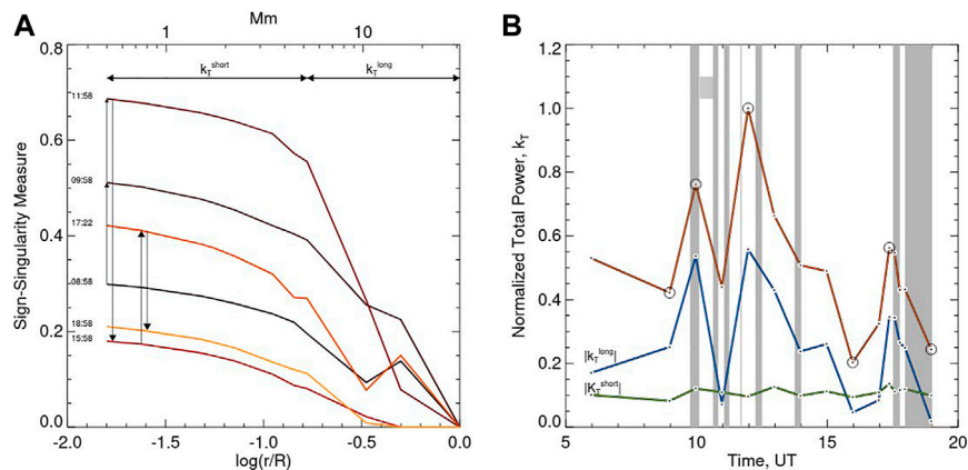
FIGURE 7 | Sign-singularity measures (A) , curves shown for selected time instances, and time variations of their parameters (B) calculated for the twist maps shown in Figure 4 . In the (A) the arrows indicate direction of the evolution of these measures, while the time stamps are shown to connect these curves to the corresponding images in Figure 4 . The two-sided arrows mark linear intervals used to calculate the cancellation exponent, k_T^{\text{short}} , and the slope of the long range end of the measure, k_T^{\text{long}} . (B) shows time variations of the total power (brown) calculated for each measure shown in the (A) , as well as the corresponding cancellation exponent ( k_T^{\text{short}} , green) and the slope ( k_T^{\text{long}} , blue). The data points indicated by circles are those that correspond to the measures in the left plot. The vertical strips indicate the start time and the duration of AIA 17.1 nm brightenings and the X1.2 flare (18:00–19:00 UT) associated with the AR filament and the horizontal bar between 10:07 and 10:37 UT marks the timing of a M7.2 flare that occurred in the south-east part of the AR.
