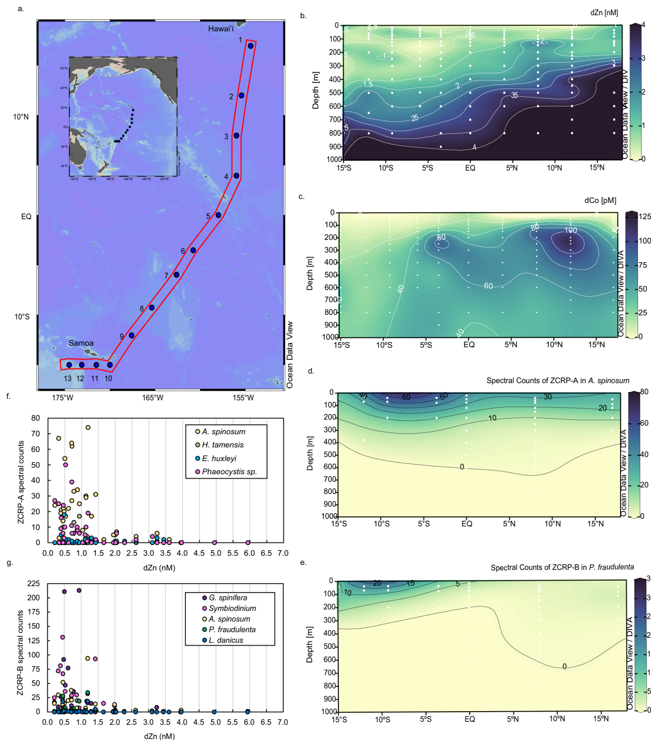
Fig. 6 Metaproteomic detection of ZCRP homologs in the Southern Pacific. a Transect sampled for dissolved Zn and metaproteomics during the KM1128 METZYME research expedition on the R/V Kilo Moana October 1–25, 2011 from O‘ahu, Hawai‘i to Apia, Samoa, in the tropical South Pacific. b The concentration of total dissolved Zn and c the concentration of total dissolved Co measured in the upper 1000 m in color scale along the METZYME transect. d Total spectral counts of the ZCRP-A homolog in the dinoflagellate Azadinium spinosum and e total spectral counts of the ZCRP-B homolog in the diatom Pseudo-nitzschia fraudulenta and measured in the upper 1000 m in color scale along the METZYME transect. f Total spectral counts of ZCRP-A homologs detected in the dinoflagellate A. spinosum , the diatom H. tamensis , and the haptophytes E. huxleyi , and Phaeocystis sp. compared to total dissolved Zn concentration. g Total spectral counts of ZCRP-B homologs detected in the dinoflagellates G. spinifera , Symbiodinium sp., A. spinosum , and in the diatoms P. fraudulenta and L. danicus compared to dZn. Detected species correspond to nearest taxonomic matches.
