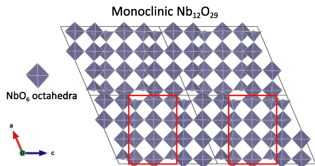
Figure 1. The crystal structure of monoclinic \text{Nb}_{12}\text{O}_{29} with unit cell framed in black outline. 4 \times 3 blocks of vertex-shared \text{NbO}_6 octahedra ( \text{ReO}_3 blocks) are framed in red outlines. Along the b direction, each 4 \times 3 block is connected to the next block by vertex-shared octahedra. Extension along the a and c directions shows blocks connecting to adjacent blocks by edge-shared octahedra (crystallographic shears).
