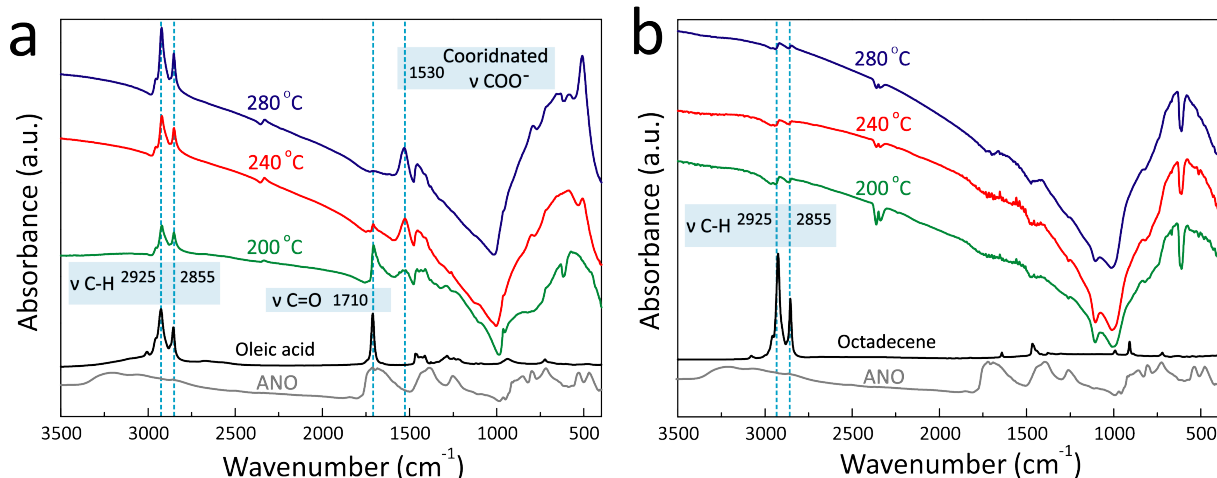
Figure 3. (a, b) FT-IR spectra of ANO, oleic acid, octadecene, and aliquots collected at 200 °C, 240 °C, and 280 °C during the nanocrystal synthesis using oleic acid and octadecene as solvents, respectively. In the spectra, peaks at 2925 and 2855 \text{cm}^{-1} correspond to the stretching of C-H bond, peak at 1710 \text{cm}^{-1} correspond to the stretching of C=O bond, and peak at 1530 \text{cm}^{-1} correspond to the asymmetric stretching of coordinated \text{COO}^- bond.
