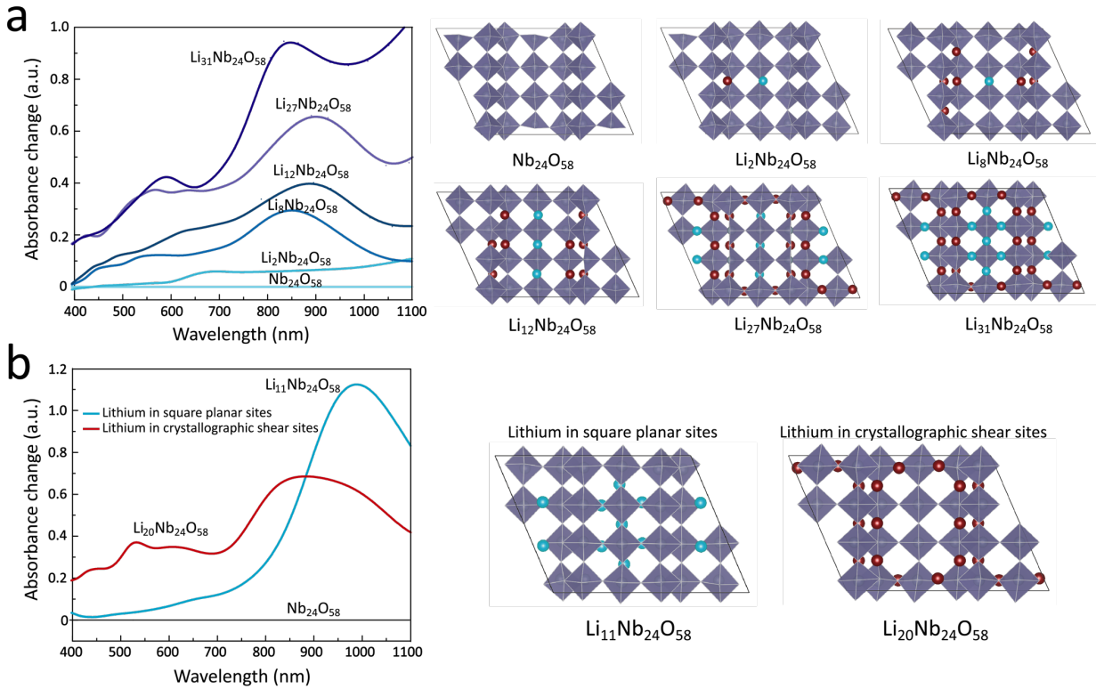
Figure 5. (a) Calculated absorbance spectra for lithiated monoclinic \text{Nb}_{12}\text{O}_{29} structures relative to the un-lithiated monoclinic \text{Nb}_{12}\text{O}_{29} and the corresponding simulated structures. Color scheme on right: \text{NbO}_6 octahedra (blue-grey), Li in square planar sites (cyan) and Li in crystallographic shear sites (dark red). (b) Absorbance spectra for lithiated monoclinic \text{Nb}_{12}\text{O}_{29} relative to the un-lithiated monoclinic \text{Nb}_{12}\text{O}_{29} with Li only in the crystallographic shear sites or the square planar sites.
