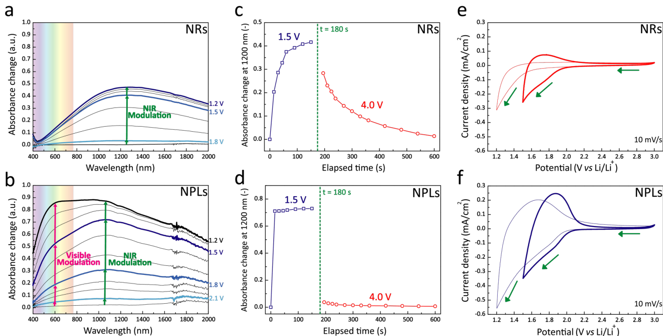
Figure 4. Spectroelectrochemical characterization of the ligand-stripped monoclinic \text{Nb}_{12}\text{O}_{29} NR and NPL films in 1 M Li-TFSI/TG. (a, b) Absorbance spectra of the nanocrystal films reduced at designated potential (vs. \text{Li/Li}^+ ) for 2 min by chronoamperometry. The interval between each spectrum is 0.1 V and the absorbance change is the difference from the OCP state to the reduced states at various potentials. (c, d) Dynamic absorbance change of the nanocrystal films at 1200 nm. The films were first reduced at 1.5 V for 180 s and subsequently oxidized at 4.0 V for 420 s by chronoamperometry. (e, f) Cyclic voltammograms of the nanocrystal films at a scan rate of 10 mV/s. For these measurements, the 5 th cycle of the cyclic voltammogram was collected to assure the films had reached stabilization.
