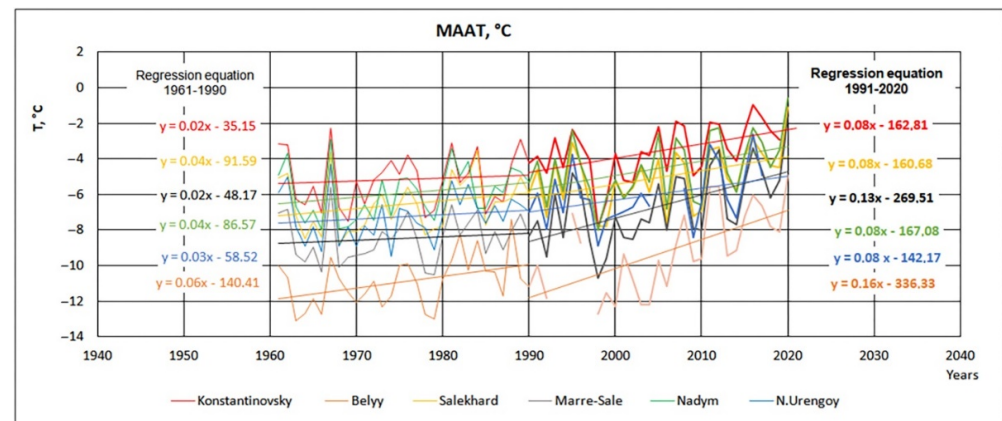
Figure 2. Changes in mean annual air temperature at weather stations in the western sector of the Russian Arctic.
