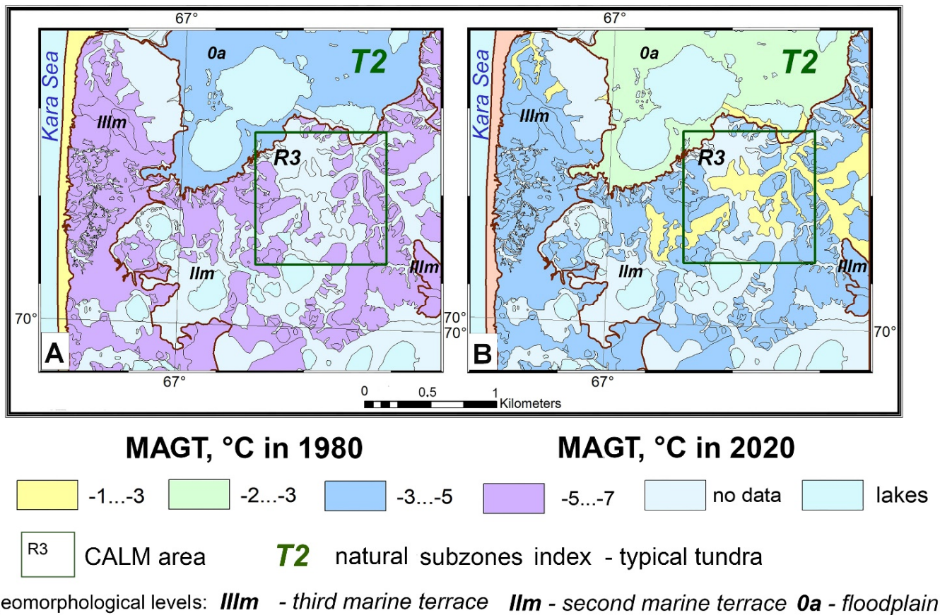
Figure 7. Changes in the mean annual ground temperature for two time intervals, Western Yamal, Marre-Sale station, typical tundra: (A) in the 1980s and (B) the modern period, 2020.
