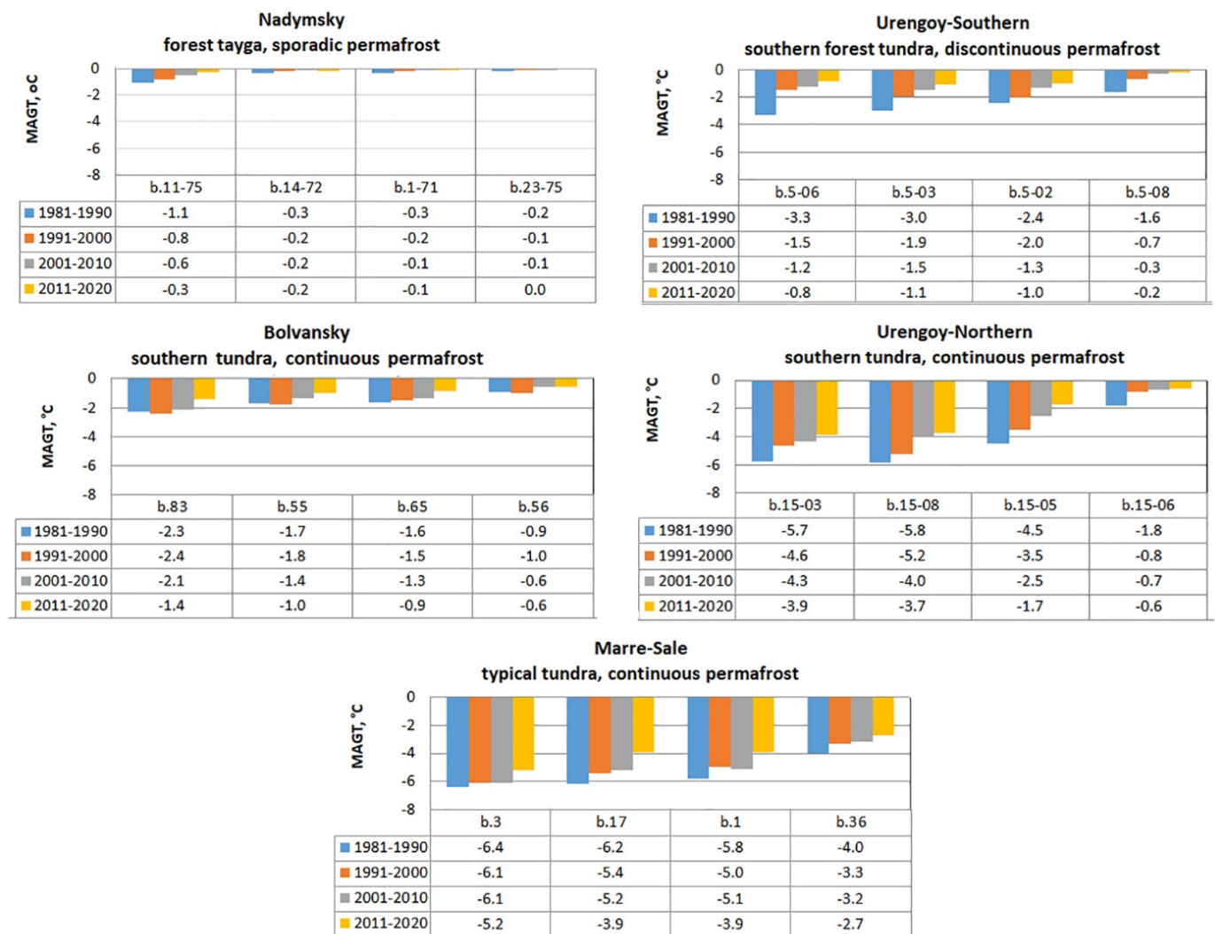
Figure 6. Mean annual ground temperature in boreholes averaged over decades at a depth of 10 m in typical cryogenic landscapes at geocryological stations.
