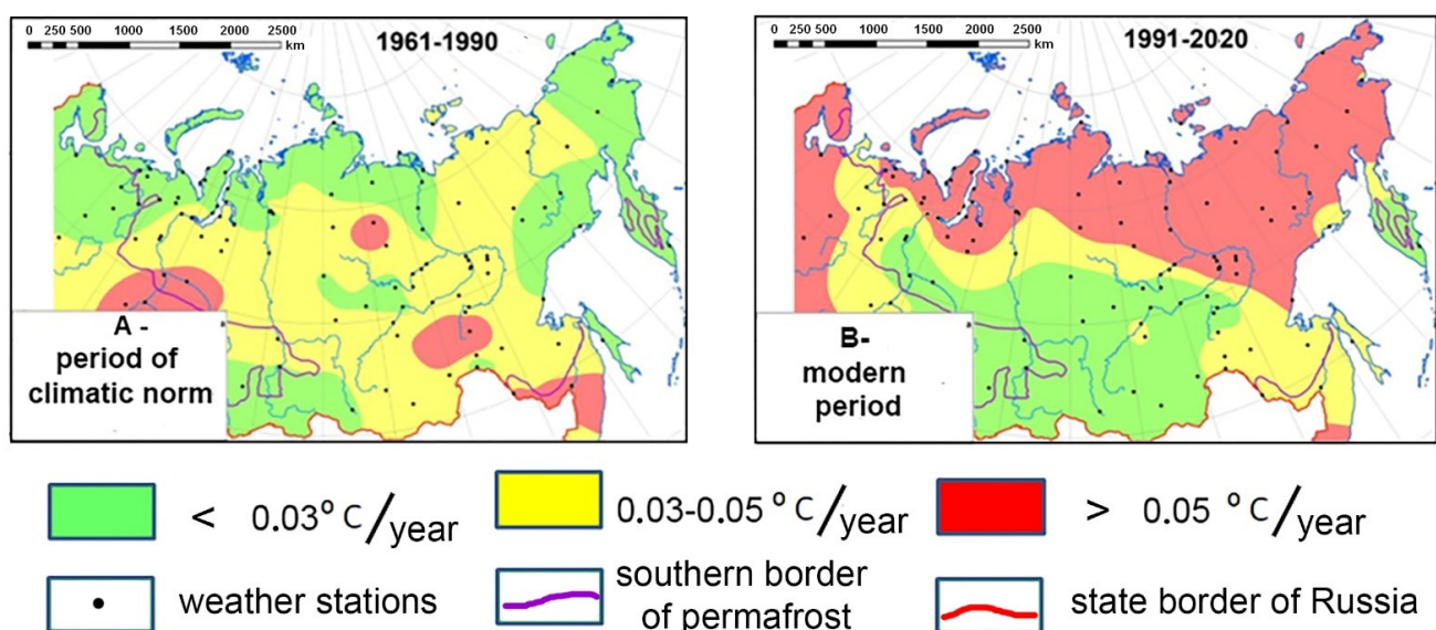
Figure 4. Spatial and temporal changes in the trend of mean annual air temperature in the Russian cryolithozone.
