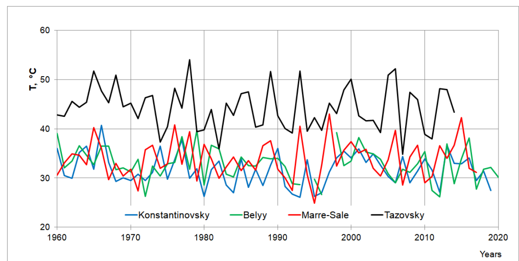
Figure 3. Changes in the annual amplitude of air temperature by weather stations in northern Russia.
