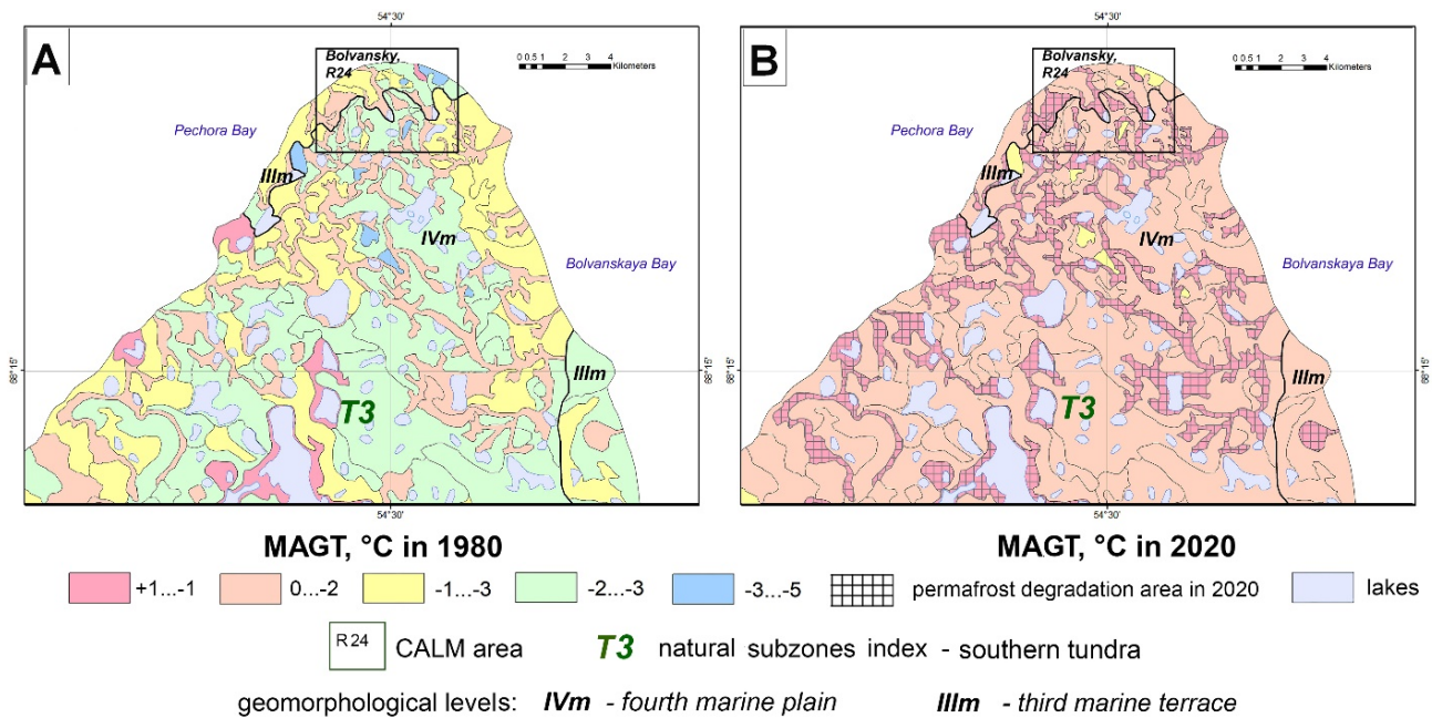
Figure 8. Changes in the mean annual ground temperature in southern tundra of the Russian European North for two time intervals: (A) in the 1980s and (B) the modern period, 2020.
