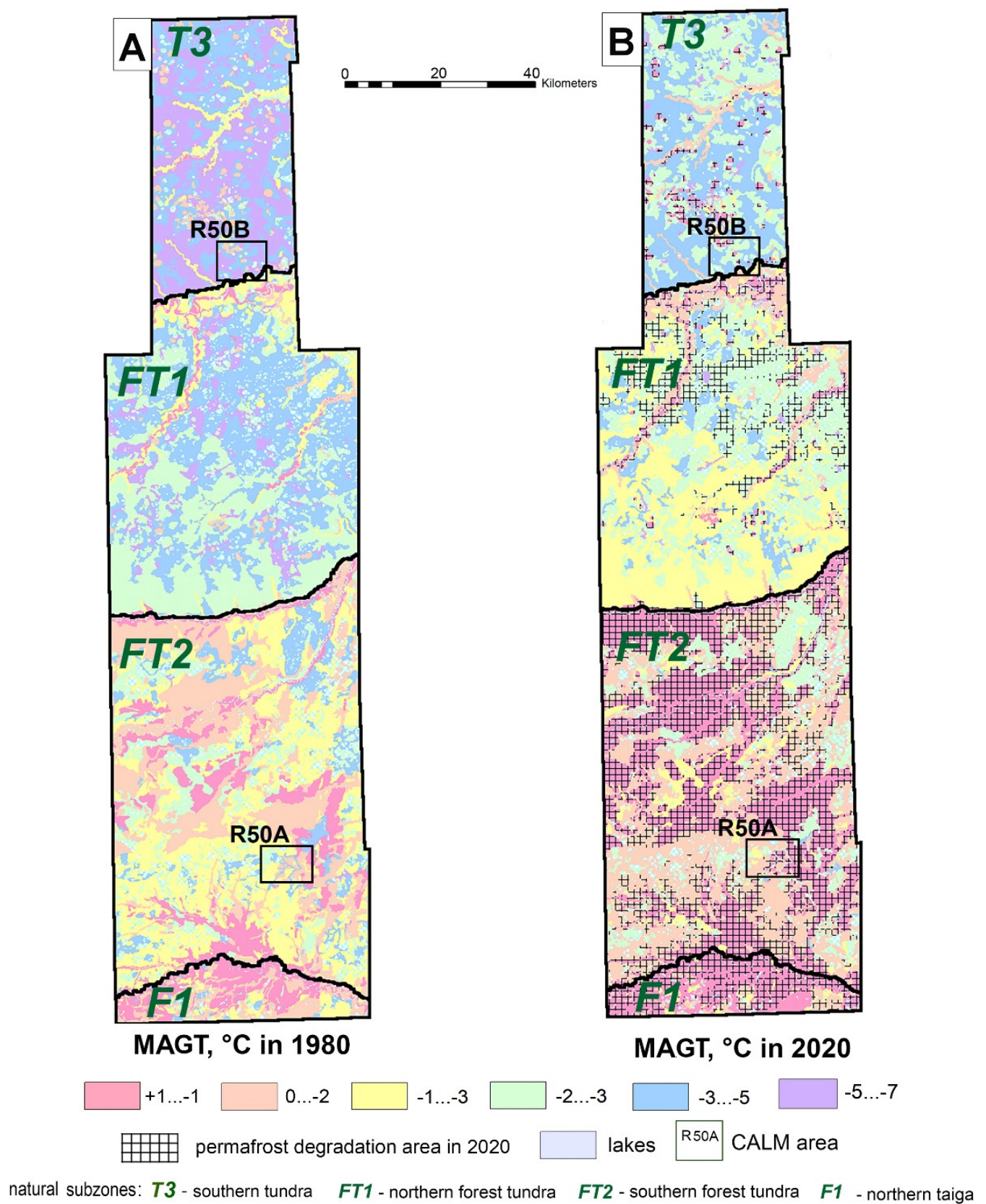
Figure 9. Changes in the mean annual ground temperatures for two time intervals: (A) the 1980s, and (B) the modern period, 2020. North of Western Siberia, the territory of the Urengoy field, transect from northern taiga to southern tundra.
