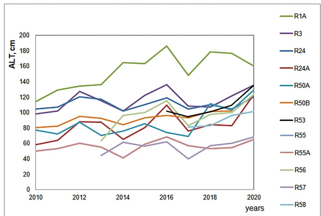
Figure 5. Interannual variability of average thaw depth at CALM sites [46].
