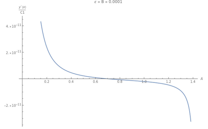
FIG. 3. The dependence of C_1^{-1}y'(x) on the parameters A and B .
