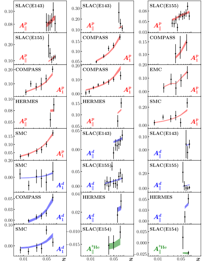
FIG. 2. Comparison of A_{||} and A_1 data (black) at x < 0.1 and Q^2 \in [1.73, 19.70] \text{ GeV}^2 with the JAMsmallx fit: proton (red), deuteron (blue), and ^3\text{He} (green).
