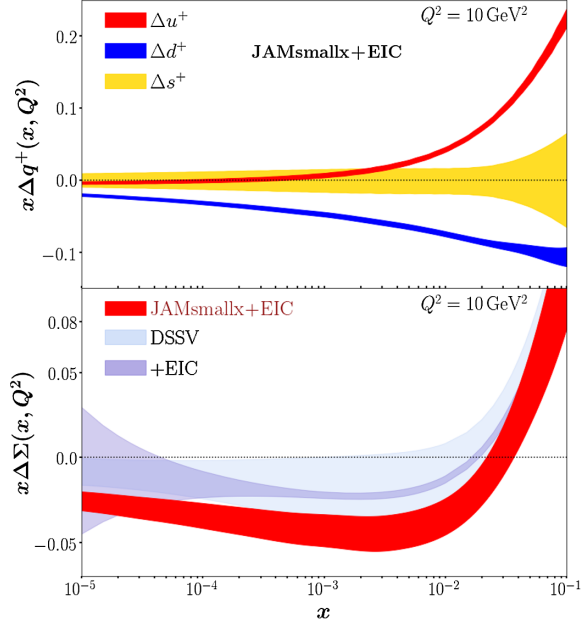
FIG. 5. Top: fitted helicity PDFs x\Delta q^+(x, Q^2) from the current JAMsmallx fit to existing polarized DIS data and EIC pseudodata for A_{||} and A_{PV} at x < 0.1 . Bottom: the result for x\Delta\Sigma(x, Q^2) from the same fit (red), compared with that from the DSSV analysis with [56] (light purple) and without [54,55] (light blue) the EIC pseudodata.
