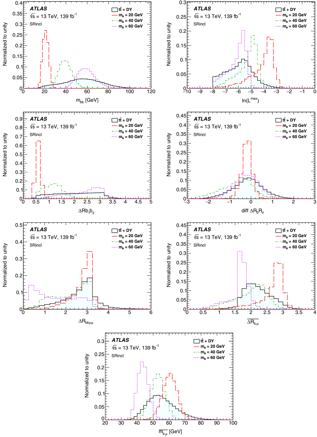
FIG. 1. Kinematic variables used as inputs to the BDT training. From top left to bottom right: m_{bb} , \ln(L^{\max}) , \Delta R_{b_1 b_2} , \text{diff} \Delta R_{b_1} R_{b_2} , \Delta R_{bb\mu\mu} , \Delta R_{b,\mu} , m_{b,\mu} . The variables are plotted in SRincl. All the distributions are normalized to unit area. The background histogram is the sum of the t\bar{t} and DY event templates, combined in the proportions extracted from the background validation fit described in Sec. VII.
