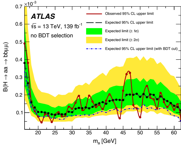
FIG. 11. Upper limits on B(H \rightarrow aa \rightarrow bb\mu\mu) at 95% CL, with no BDT selection applied, as a function of the signal mass hypothesis. The dash-dotted blue line indicates the expected limit set in the analysis with the BDT selection. Black and red dots show masses for which the hypothesis testing was done. Between these points, the limits are interpolated and may not be fully representative of the actual sensitivity.
