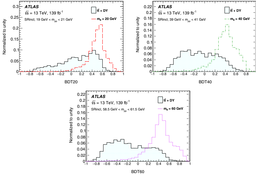
FIG. 2. Three \text{BDT}_{m_a} distributions, BDT20, BDT40, and BDT60, plotted in the m_{\mu\mu} windows of SRincl, as indicated in the figures. The distributions are normalized to unit area. The background histogram is the sum of the t\bar{t} and DY event templates, combined in the proportions extracted from the background validation fit described in Sec. VII.
