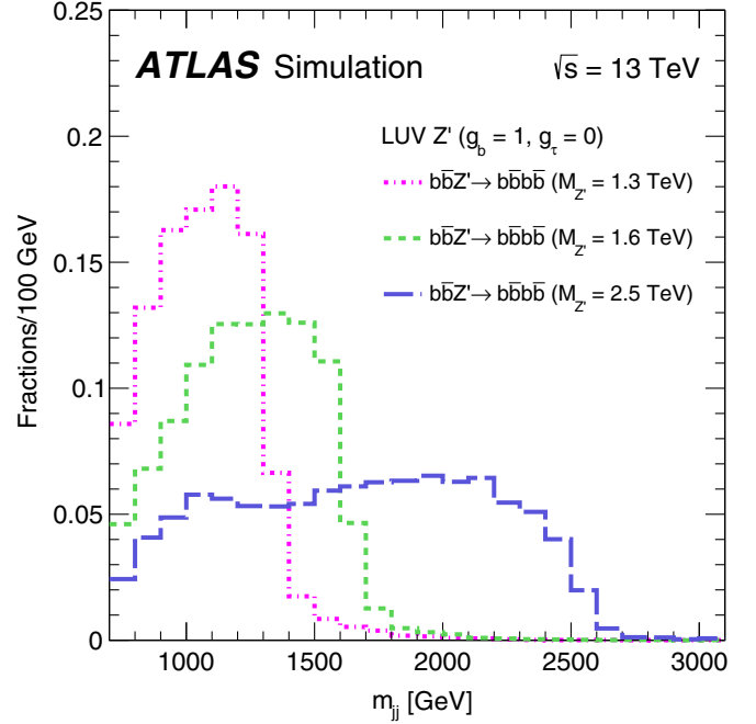
FIG. 2. m_{jj} distributions of three benchmark LUV Z' mass points, 1.3 TeV, 1.6 TeV, and 2.5 TeV after applying the full signal region selections, normalized to unity.
