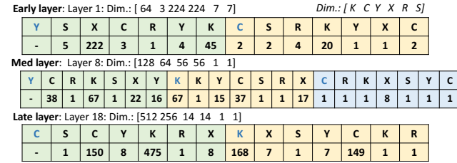
Figure 7: GAMMA's found mapping of early, medium, and late layer
