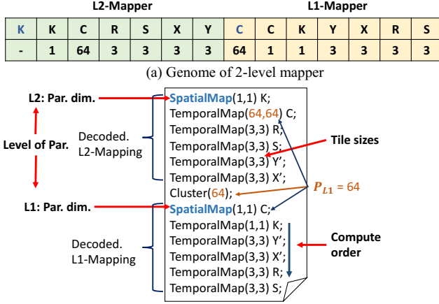
(b) Decoded 2-level genome in cost model (MAESTRO) 's description Figure 4: (a) GAMMA's description of a 2-level mapper and (b) its decoded description for cost model (MAESTRO) of a NVDLA-like [1] 2-level mapper.
