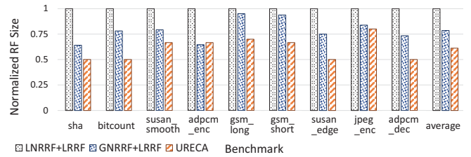
Fig. 8. Managing all variables in the unified RF reduces register requirement significantly as compared to CGRA managing the variables in separate RFs.
