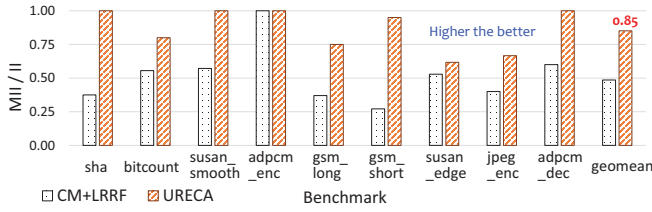
Fig. 5. Managing all variables within local unified RF achieves II close to Minimum II (MII) as compared to CGRA accessing constant memory.
