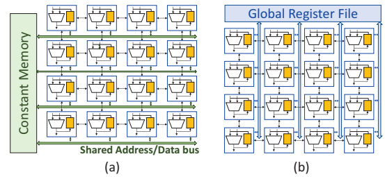
Fig. 2. CGRAs manage recurring variables in local rotating RFs. For nonrecurring values, CGRA accesses (a) on-chip memory (b) a global RF; each PE is connected to global RF through column-wise bus structure
