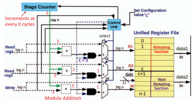
Fig. 3. Unified RF is a regular register file that can be split in rotating and nonrotating sections. Compiler configures RF through a machine instruction.
