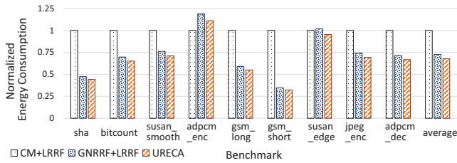
Fig. 7. Normalized energy consumption for CGRA with unified RF and for CGRA managing nonrecurring values in global RF when compared to the approach of accessing nonrecurring variables from memory.
