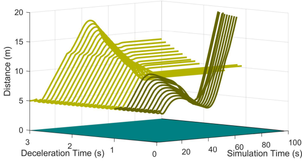
Figure 12: Merge scenario - CAVs distance remains greater than a threshold for all cases where the CAV with advantage stops before entering the merge (Yellow) or after the merge (dark green).
