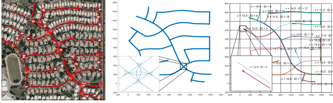
Figure 8: A snapshot of a map retrieved from the OpenStreetMap (left), its corresponding directed graph in MATLAB (middle) and a scenario with randomly spawned vehicles on the map (Right).
