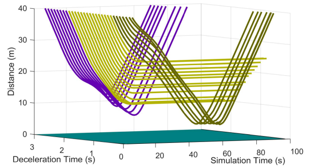
Figure 11: Brute-force evaluation of an intersection scenario. CAVs distance is always greater than a threshold regardless of the deceleration time of the CAV with the advantage –if it stops before entering the conflict zone (dark green), inside the conflict zone (yellow), or after the conflict zone (blue).
