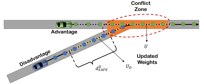
Figure 7: Weights of the edges on the path of the other CAV and edges on path of the ego CAV are updated to account for the presence of other CAVs as well as the conflict zone and the required safe distance.
