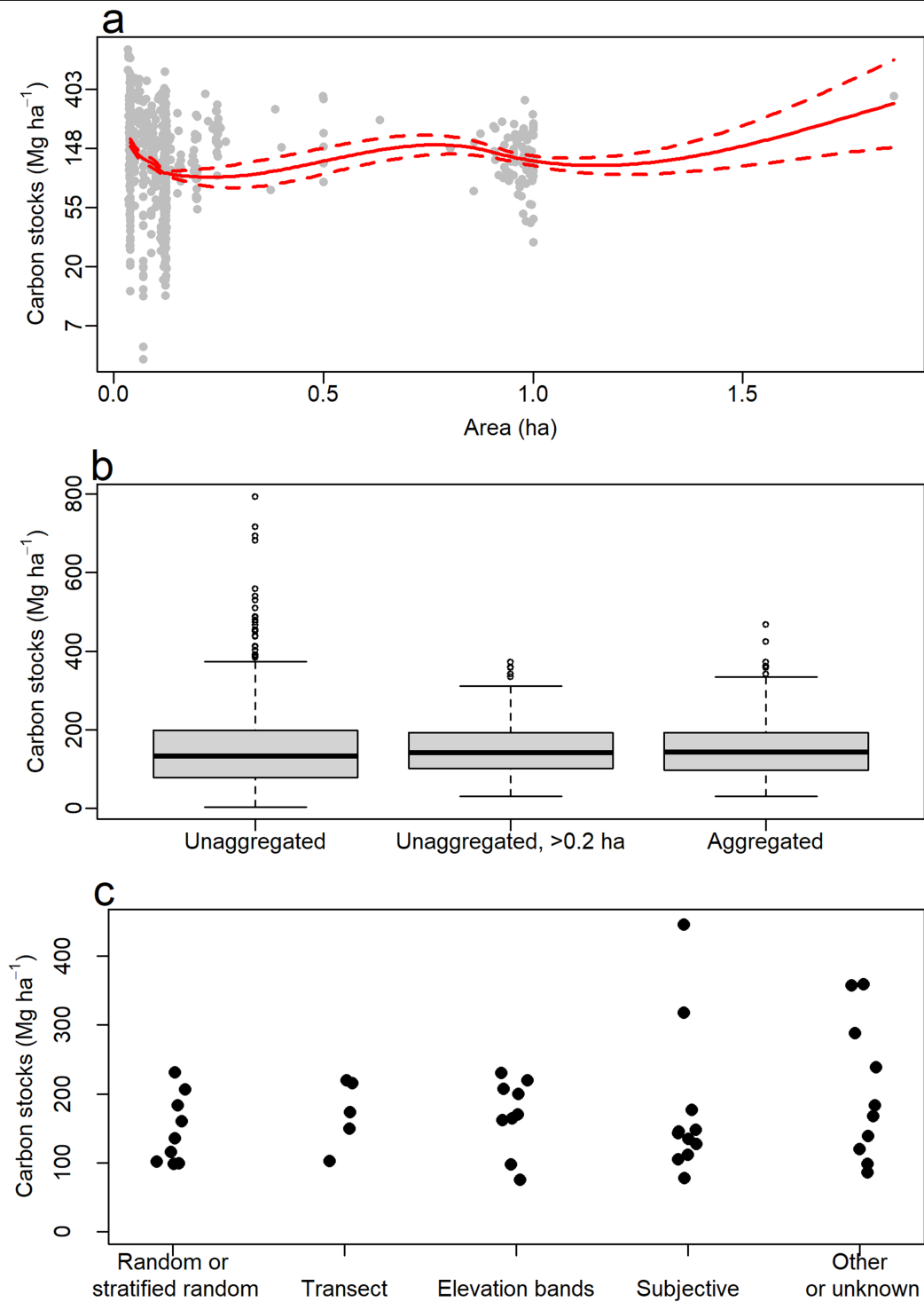
Extended Data Fig. 2 | Effect of plot area, aggregation procedure and plot design on estimates of AGC stocks across the AfriMont plot network. a , Relationship between AGC stocks and plot area of plots before aggregation. The red line shows the fit of a locally weighted regression model (span 0.75) relating these variables, with dashed lines showing the standard errors. b , Variation in AGC stocks using either all plots before aggregation (unaggregated), plots before aggregation but excluding those <0.2 ha (unaggregated, >0.2 ha) or the aggregated plots used in the main analyses (aggregated). c , Effects of plot design on AGC stocks (each site represents one
