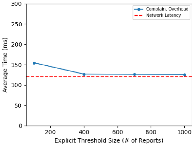
Fig. 2: Average complaint time as a function of the threshold with n = 1,000,000 complaints per epoch. Complaint time is measured as the average of 100 samples and has a variance of less than 5ms. Network latency shows the minimum latency required to transmit 3 sequential messages over the network, a lower bound on complaint time.
