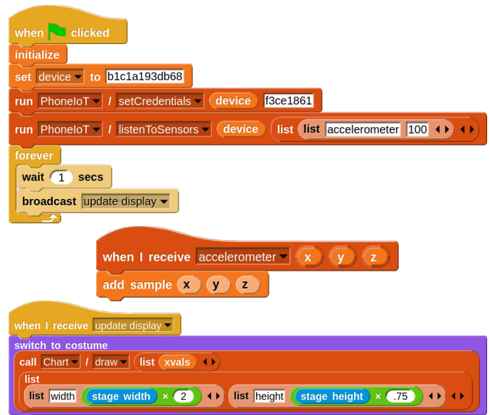
Fig. 7. Code running the accelerometer plotter project. The “add sample” custom block maintains three lists (xvals, yvals, zvals). The “update display” script is only shown for the x sprite.
