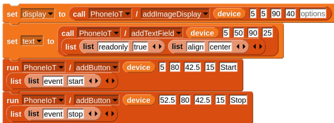
Fig. 5. Blocks used to set up the PhoneIoT device display for the GPS tracker.
