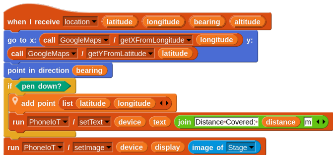
Fig. 6. Location message handler. It reads live GPS data from the mobile device, plots the track on a map on the stage, and sends the map/track back as an image to the device. Note that the “add point” custom block maintains the list of locations and computes the distance using a Google Maps RPC.
