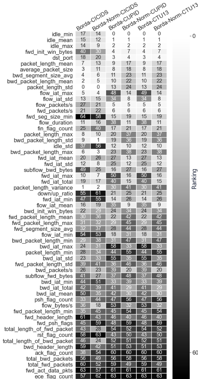
Fig. 2: Ranked features across datasets, sorted by median. A smaller value indicates a better ranking.
