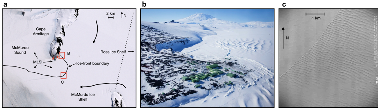
Fig. 5. (A) Landsat Image Mosaic of Antarctica (LIMA) showing the environs of Cape Armitage and the McMurdo Ice Shelf (Bindshadler and others, 2008). McMurdo Station and Scott Base are indicated by red stars on the southern tip of the cape. Approximate ice-flow directions are shown by curved arrows on the right side of image. Red boxes display the areas pictured in the oblique aerial photos of panels B and C. The scenes the oblique photos are viewing are indicated by the red boxes labeled accordingly, and the view direction for both photos is from the south looking to the north. (B) Oblique aerial photograph (looking north) of rolls along the coastline of Cape Armitage (labeled B in panel A). Rolls in the foreground are in MLSI; rolls in the distance are on the McMurdo Ice Shelf. Roughness on the top of rolls closest to coastline indicates fracture damage. (Photo provided by Anthony Powell, an artist in residence at Scott Base.) (C) Oblique aerial photograph (looking north) of rolls in the open (non-coastal) part of the McMurdo Ice Shelf at the location labeled C in panel A (from the Antarctic Map and Photograph Library, US Geological Survey). The sharp line (running upper center to lower left) between rolls and flat MLSI is the ice front of the McMurdo Ice Shelf. This photo was taken in 1959, and the area of rolls visible has since calved and been transported away as icebergs.
